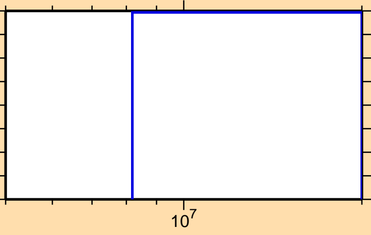
\sigma vs. E for ^{203}\text{Po}(n,\text{nd})
