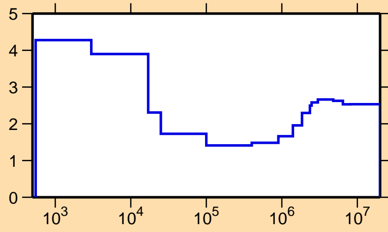
\sigma vs. E for ^{203}\text{Po}(n,\text{nonel.})
