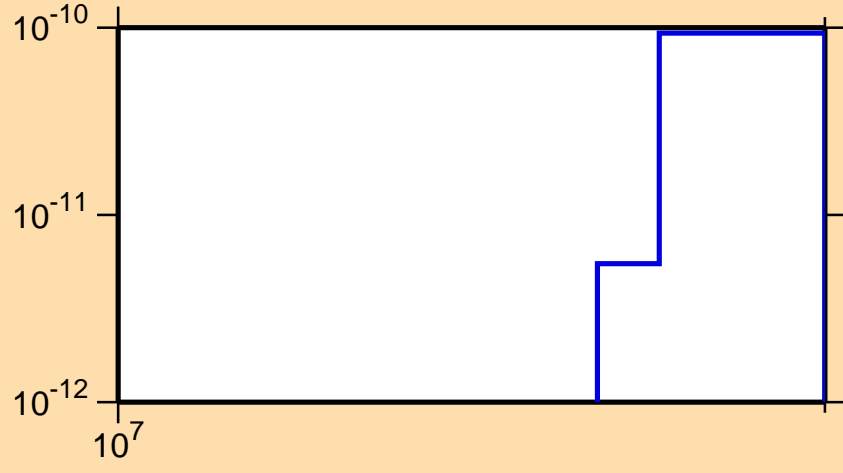
\sigma vs. E for ^{203}\text{Po}(n,\text{pt})
