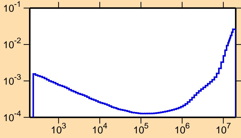
\sigma vs. E for ^{203}\text{Po}(n,\alpha)
