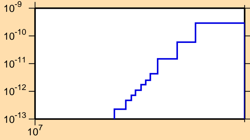
\sigma vs. E for ^{203}\text{Po}(\text{mt117})
