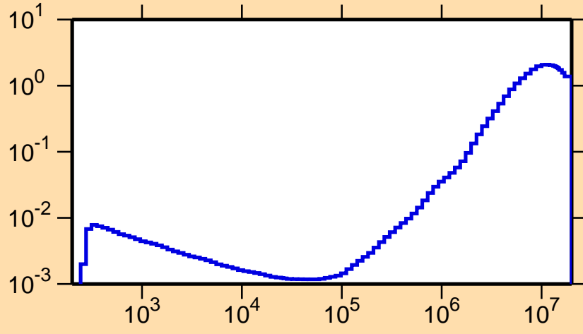
\sigma vs. E for ^{203}\text{Po}(n,\text{inel.})
