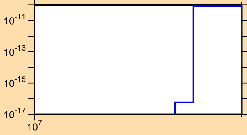
\sigma vs. E for ^{203}\text{Po}(n,3n\alpha)
