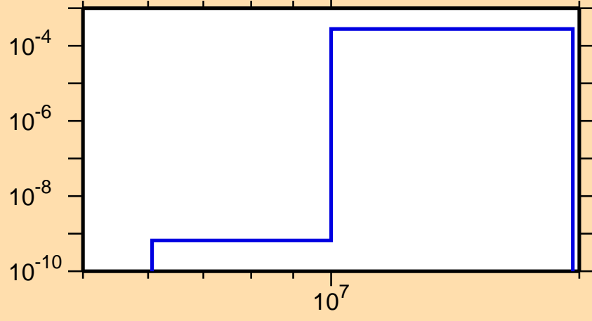
\sigma vs. E for ^{203}\text{Po}(n,t)
