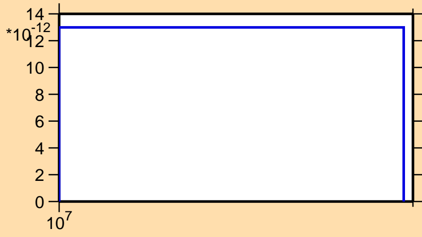
\sigma vs. E for ^{203}\text{Po}(n,\text{pd})
