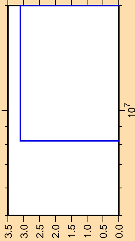
\Delta\sigma/\sigma vs. E for ^{203}\text{Po}(\text{mt } 34)
