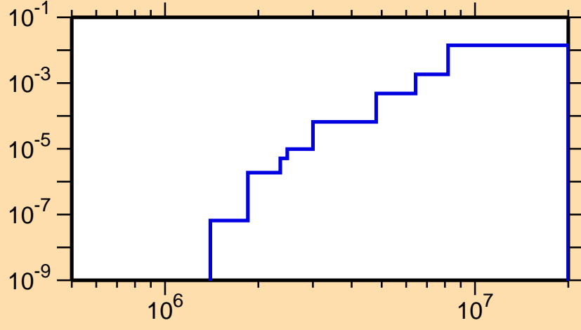
\sigma vs. E for ^{203}\text{Po}(n,n\alpha)
