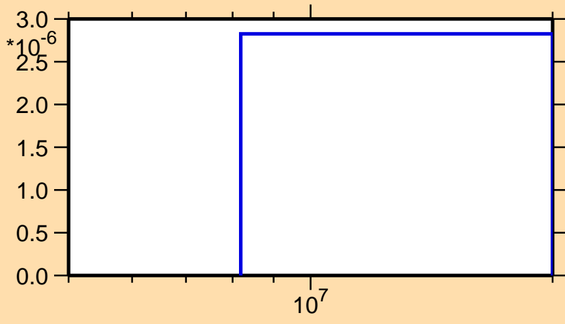
\sigma vs. E for ^{203}\text{Po}(n,3n)
