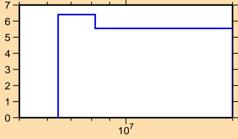
\Delta\sigma/\sigma vs. E for ^{203}\text{Po}(n,\text{nonel.})
