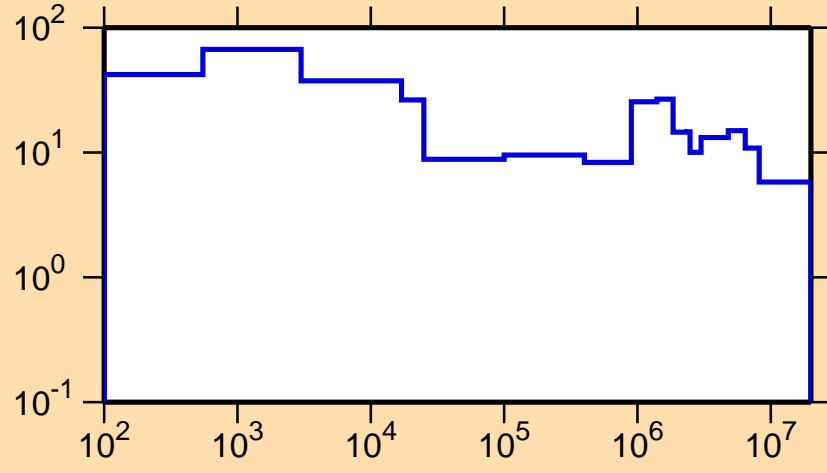
\Delta\sigma/\sigma vs. E for ^{203}\text{Po}(n, el.)
