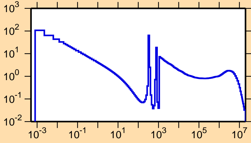
\sigma vs. E for ^{204}\text{Po}(n,\gamma)
