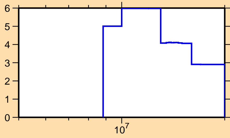
\Delta\sigma/\sigma vs. E for ^{204}\text{Po}(n,\text{tot.})
