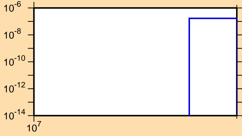
\sigma vs. E for ^{204}\text{Po}(n,3n\alpha)
