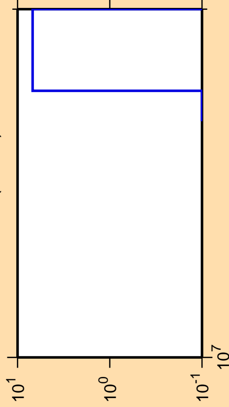
\Delta\sigma/\sigma vs. E for ^{204}\text{Po}(\text{mt } 34)
