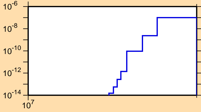
\sigma vs. E for ^{204}\text{Po}(n,\text{nd})
