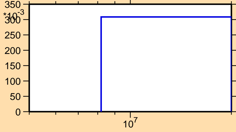
\sigma vs. E for ^{204}\text{Po}(n,2n)
