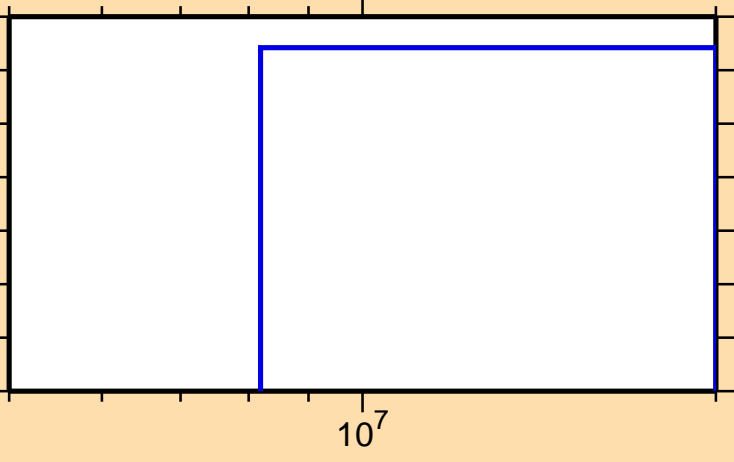
\sigma vs. E for ^{204}\text{Po}(n,nt)
