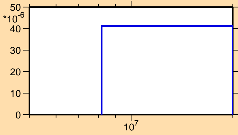
\sigma vs. E for ^{204}\text{Po}(n,t)
