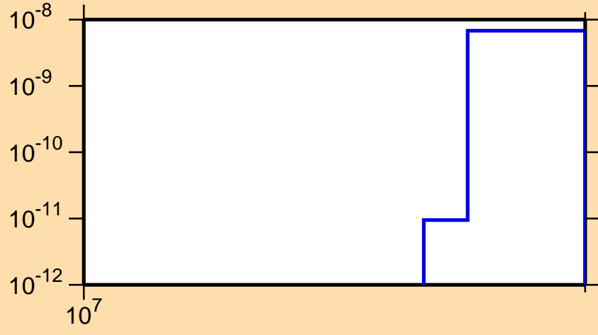
\sigma vs. E for ^{205}\text{Po}(n,nt)
