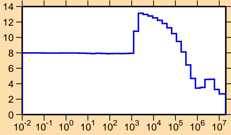
\sigma vs. E for ^{205}\text{Po}(n,\text{el.})
