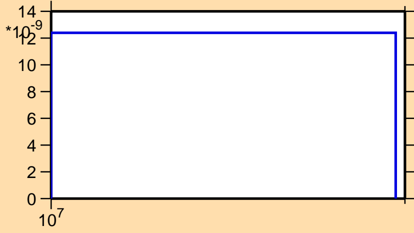
\sigma vs. E for ^{205}\text{Po}(n,3n\alpha)
