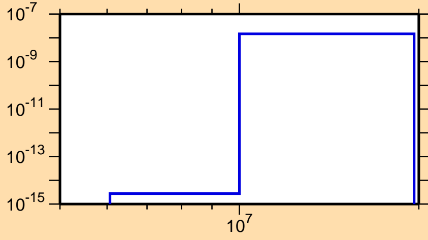
\sigma vs. E for ^{205}\text{Po}(n,\text{He}3)
