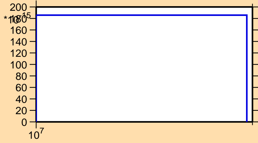
\sigma vs. E for ^{205}\text{Po} (mt 34)
