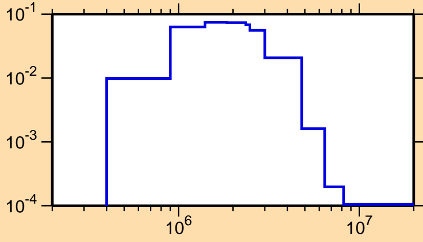
\sigma vs. E for ^{205}\text{Po}(n,n_4)
