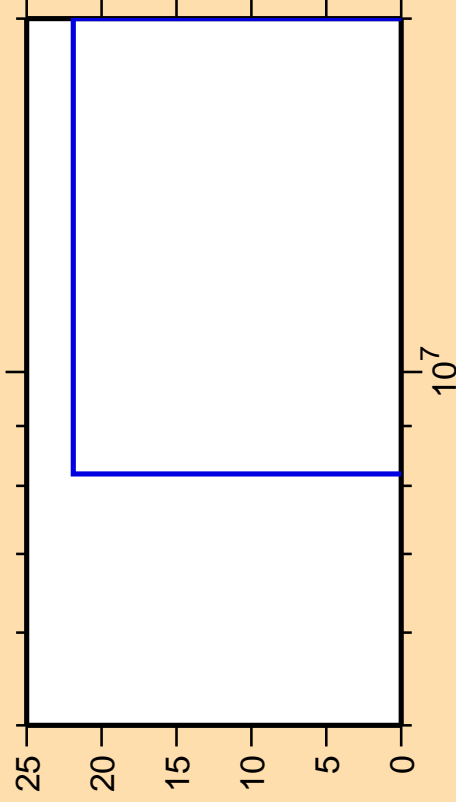
\Delta\sigma/\sigma vs. E for ^{205}\text{Po}(\text{mt117})
