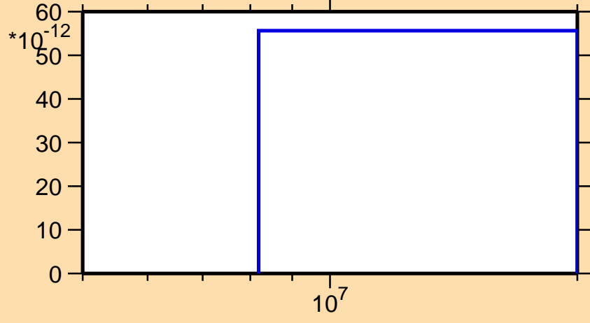
\sigma vs. E for ^{205}\text{Po}(n,nt)
