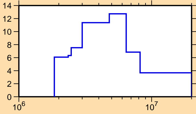
\Delta\sigma/\sigma vs. E for ^{205}\text{Po}(n,\text{tot.})
