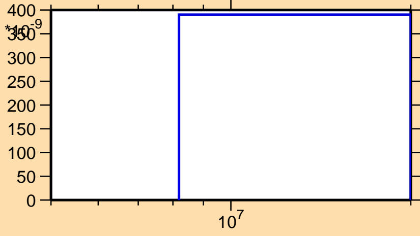
\sigma vs. E for ^{205}\text{Po}(n,2np)
