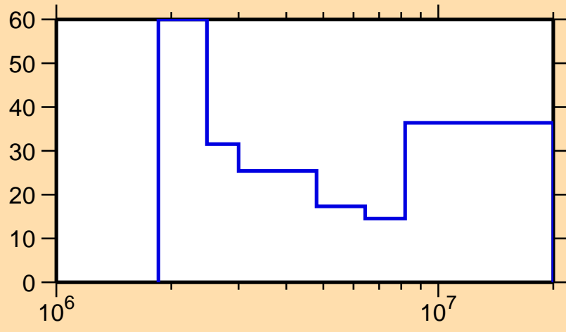
\Delta\sigma/\sigma vs. E for ^{205}\text{Po}(n,n\text{cont.})
