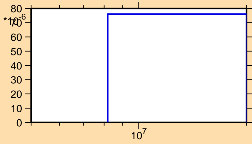
\sigma vs. E for ^{205}\text{Po}(n,3n)
