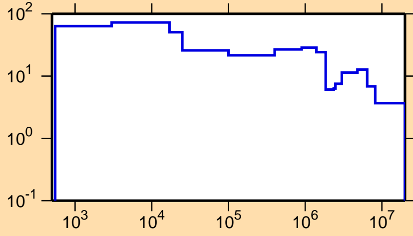
\Delta\sigma/\sigma vs. E for ^{205}\text{Po}(n,\text{tot.})
