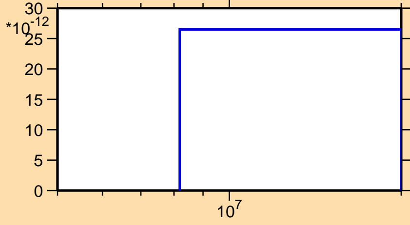
\sigma vs. E for ^{205}\text{Po}(\text{mt } 45)
