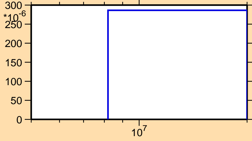
\sigma vs. E for ^{205}\text{Po}(n,2n\alpha)
