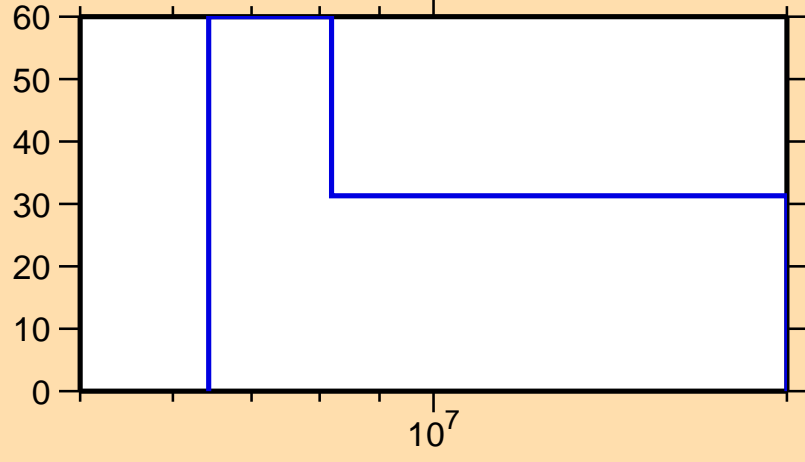
\Delta\sigma/\sigma vs. E for ^{205}\text{Po}(n,2n)
