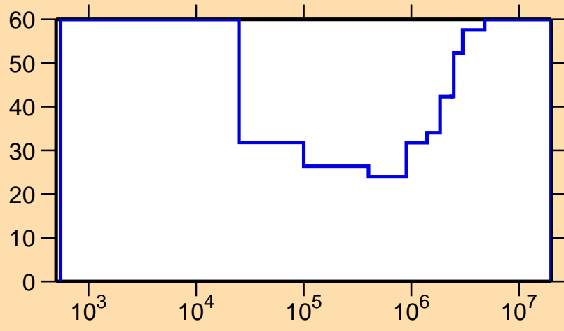
\Delta\sigma/\sigma vs. E for ^{205}\text{Po}(n,\gamma)
