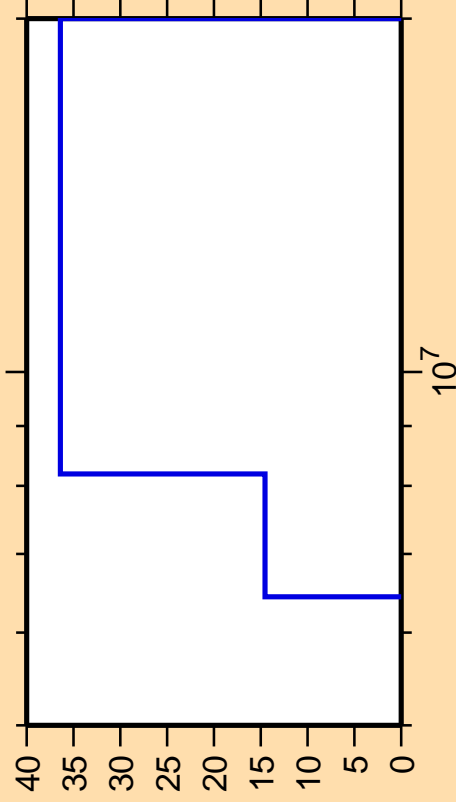
\Delta\sigma/\sigma vs. E for ^{205}\text{Po}(n,n\text{cont.})
