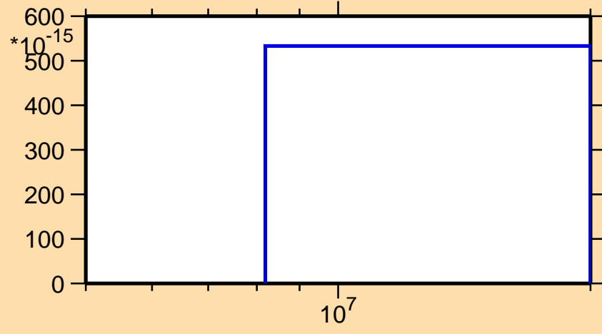
\sigma vs. E for ^{205}\text{Po}(n,\text{pt})
