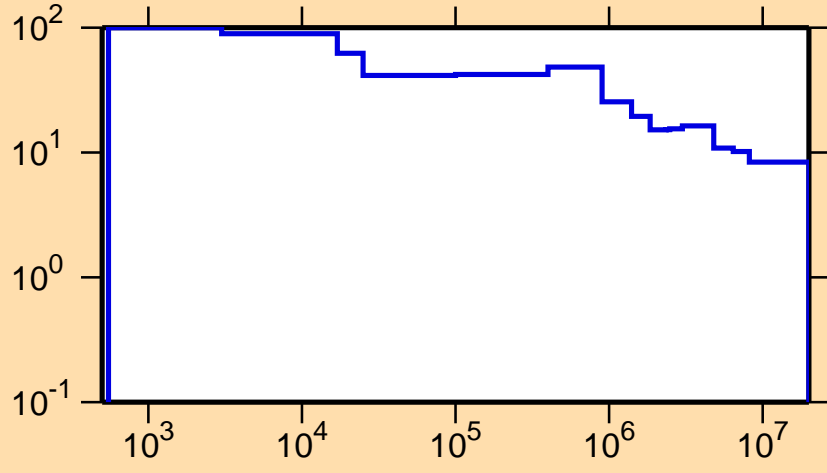
\Delta\sigma/\sigma vs. E for ^{205}\text{Po}(n,\text{nonel.})
