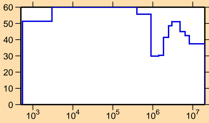
\Delta\sigma/\sigma vs. E for ^{205}\text{Po}(n,p)
