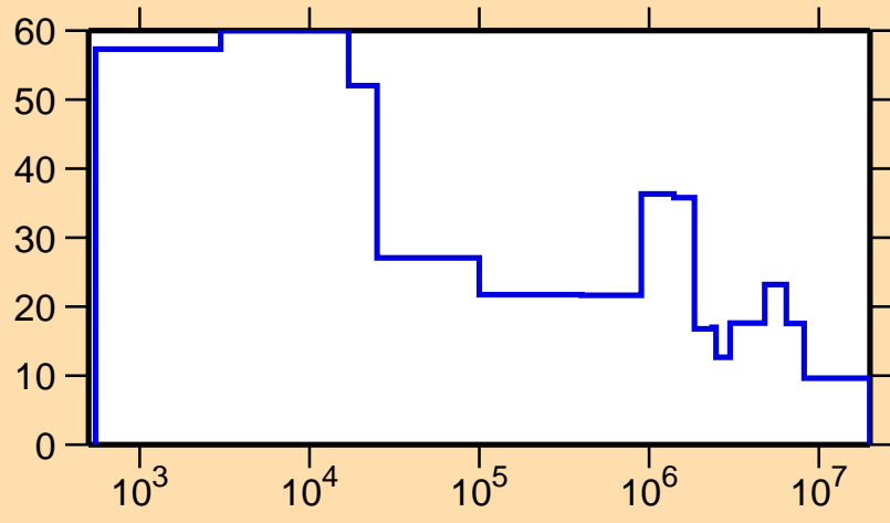
\Delta\sigma/\sigma vs. E for ^{205}\text{Po}(n,\text{el.})
