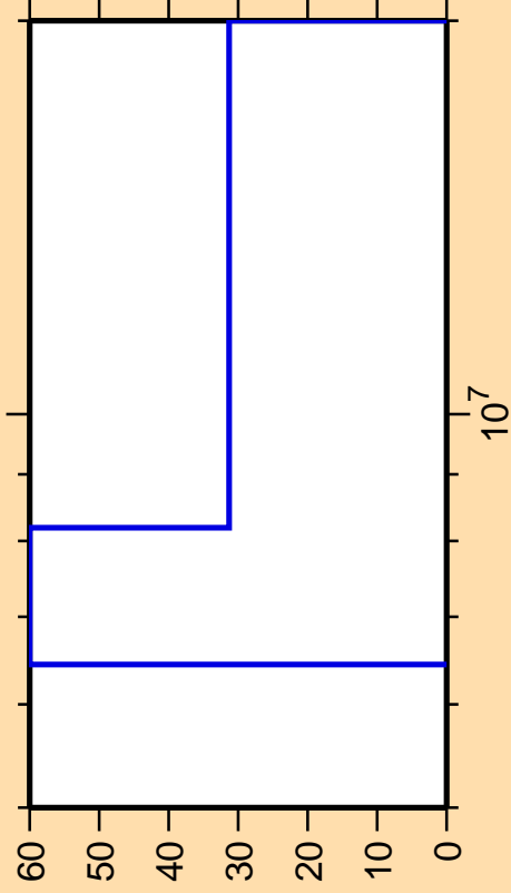
\Delta\sigma/\sigma vs. E for ^{205}\text{Po}(n,2n)
