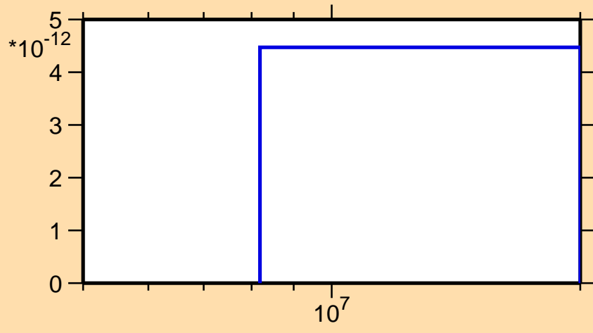
\sigma vs. E for ^{205}\text{Po}(n,\text{pd})
