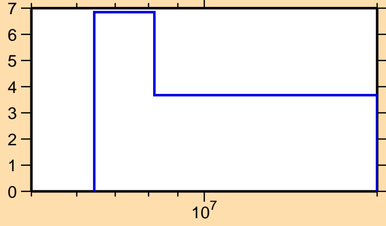
\Delta\sigma/\sigma vs. E for ^{205}\text{Po}(n,\text{tot.})
