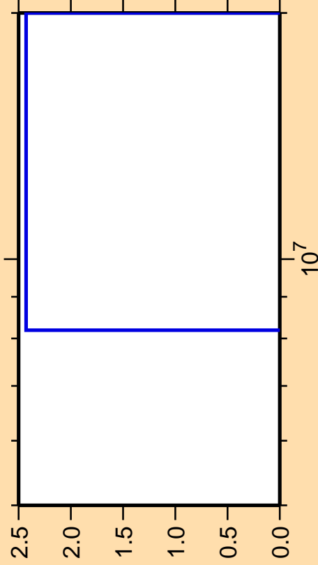
\Delta\sigma/\sigma vs. E for ^{205}\text{Po}(n,\text{pt})
