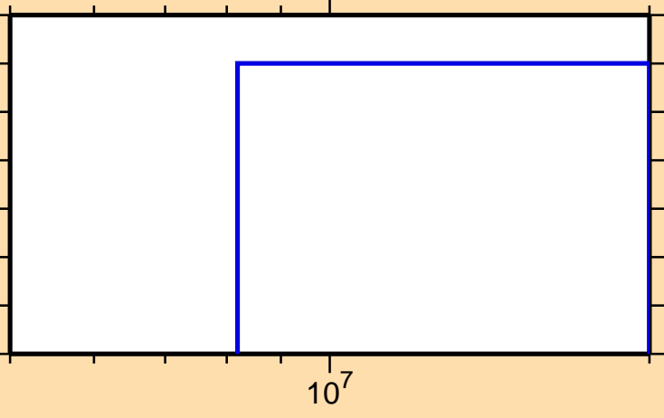
\sigma vs. E for ^{205}\text{Po}(n,\text{He}3)
