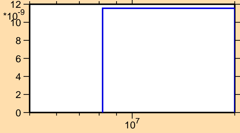
\sigma vs. E for ^{205}\text{Po}(n,3n\alpha)
