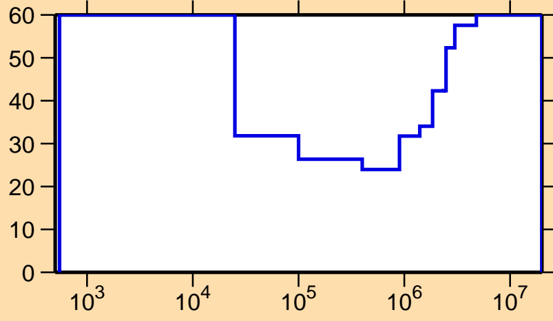
\Delta\sigma/\sigma vs. E for ^{205}\text{Po}(n,\gamma)
