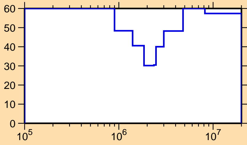
\Delta\sigma/\sigma vs. E for ^{205}\text{Po}(n,n_1)
