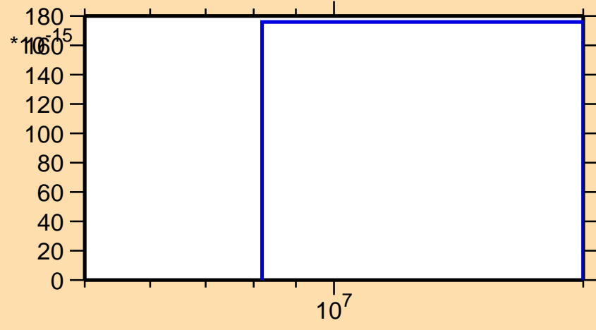
\sigma vs. E for ^{205}\text{Po}(\text{mt } 34)
