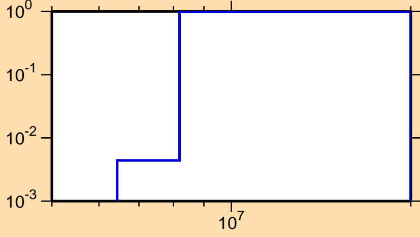
\sigma vs. E for ^{205}\text{Po}(n,2n)
