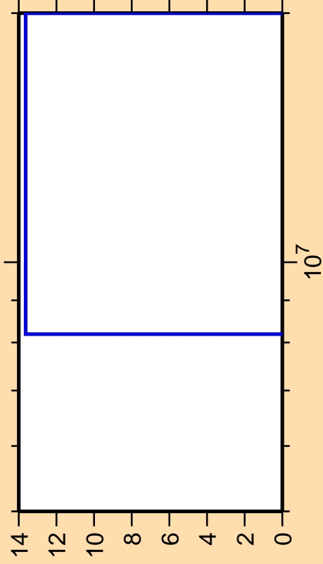
\Delta\sigma/\sigma vs. E for ^{205}\text{Po}(n,\text{pd})
