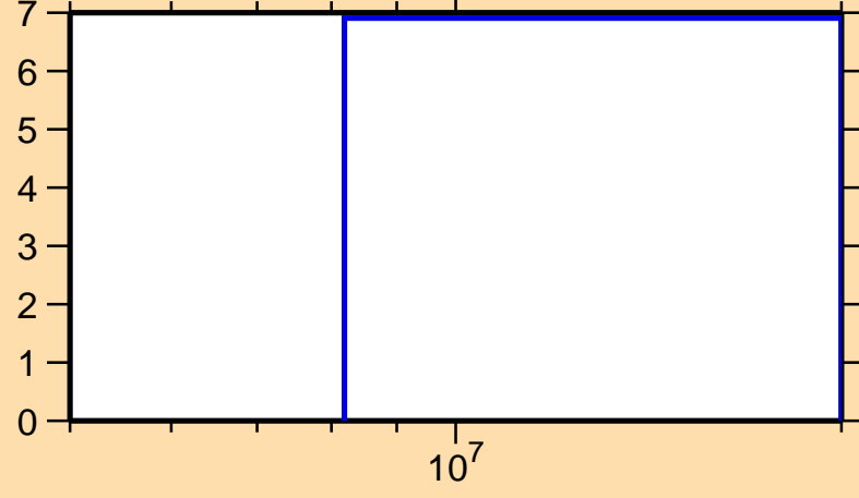
\Delta\sigma/\sigma vs. E for ^{206}\text{Po}(n,\text{el.})
