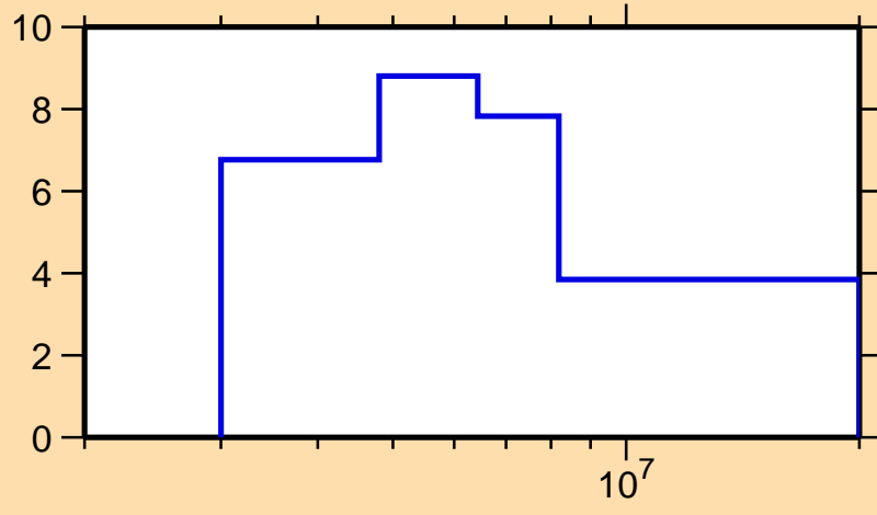
\Delta\sigma/\sigma vs. E for ^{206}\text{Po}(n,\text{tot.})
