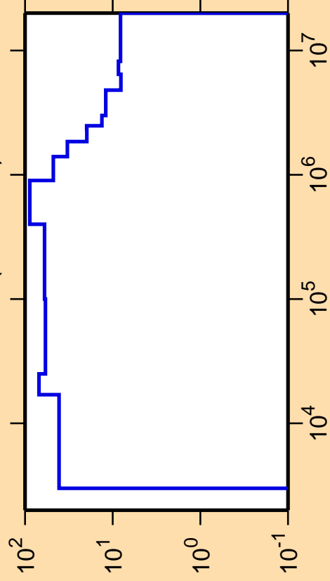
\Delta\sigma/\sigma vs. E for ^{206}\text{Po}(n,\text{nonel.})
