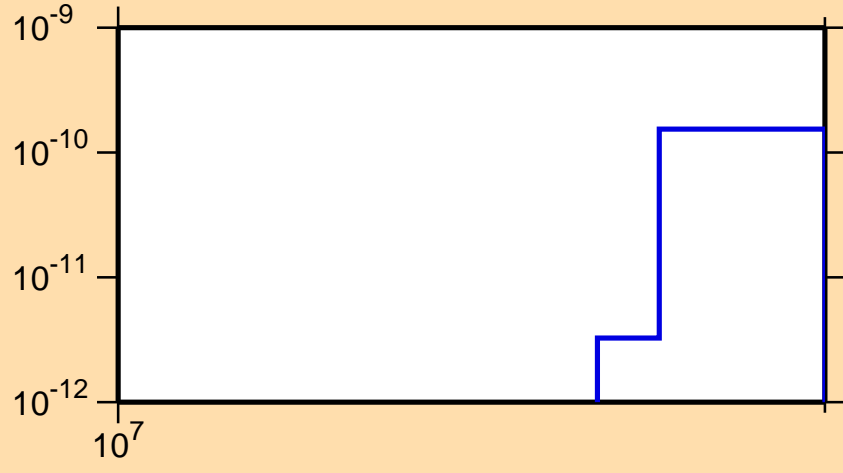
\sigma vs. E for ^{207}\text{Po}(n,\text{pt})
