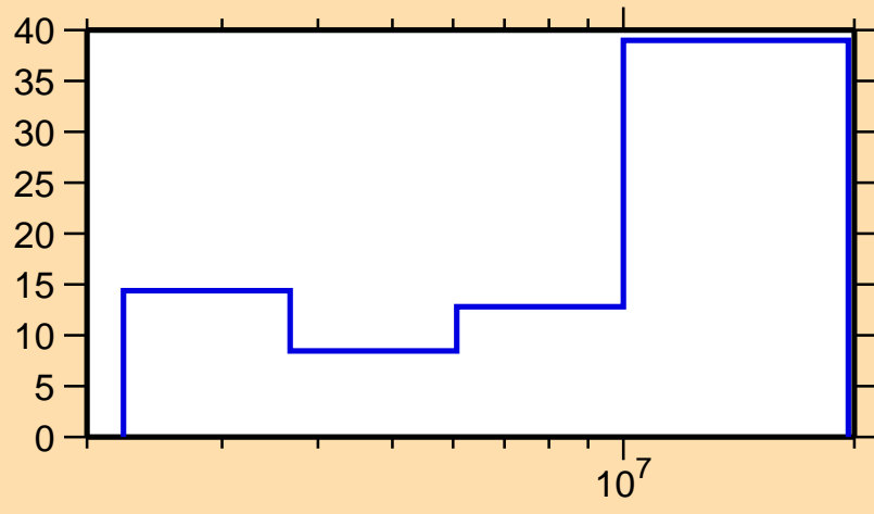
\Delta\sigma/\sigma vs. E for ^{207}\text{Po}(n,n\text{cont.})
