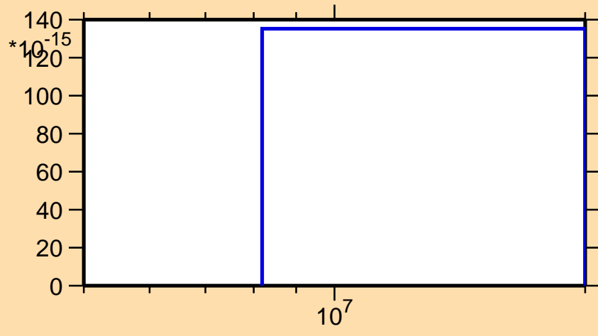
\sigma vs. E for ^{207}\text{Po}(\text{mt } 34)
