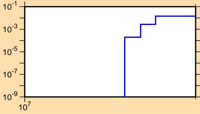
\sigma vs. E for ^{207}\text{Po}(n,3n\alpha)
