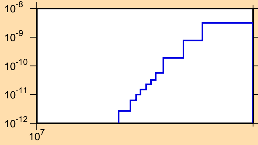
\sigma vs. E for ^{207}\text{Po}(\text{mt117})
