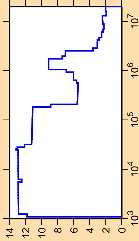
\Delta\sigma/\sigma vs. E for ^{207}\text{Po}(n,\text{nonel.})
