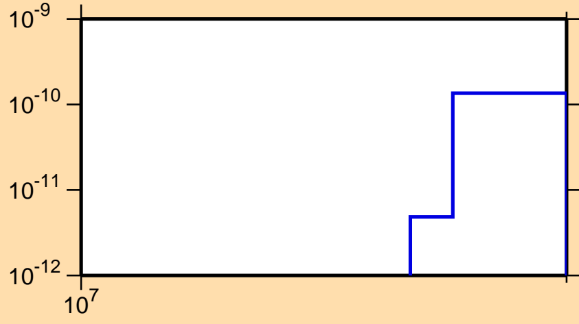
\sigma vs. E for ^{207}\text{Po} (mt 34)
