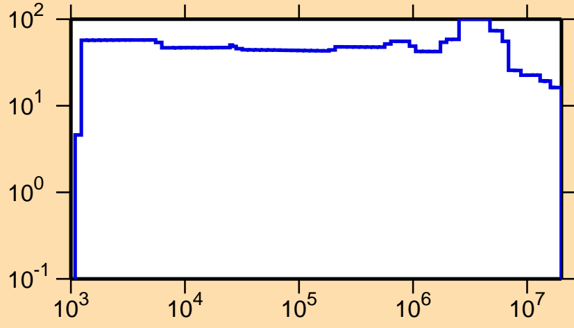
\Delta\sigma/\sigma vs. E for ^{207}\text{Po}(n,p)
