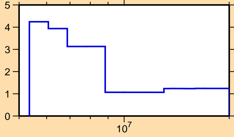
\Delta\sigma/\sigma vs. E for ^{207}\text{Po}(n,\text{el.})
