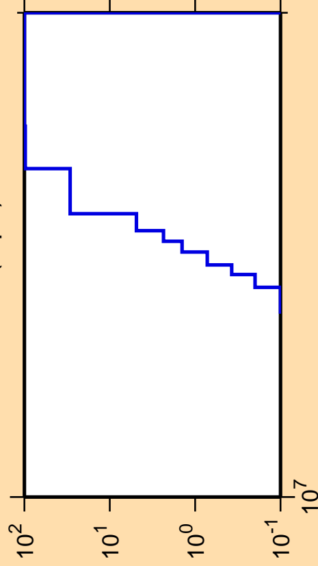
\Delta\sigma/\sigma vs. E for ^{207}\text{Po}(n,\text{pd})
