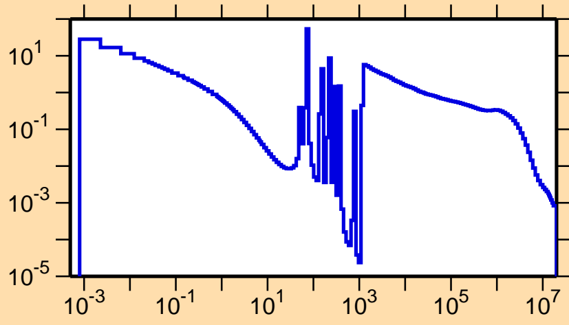
\sigma vs. E for ^{207}\text{Po}(n,\gamma)
