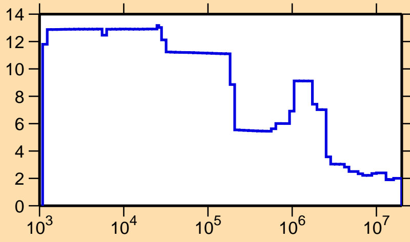
\Delta\sigma/\sigma vs. E for ^{207}\text{Po}(n,\text{nonel.})
