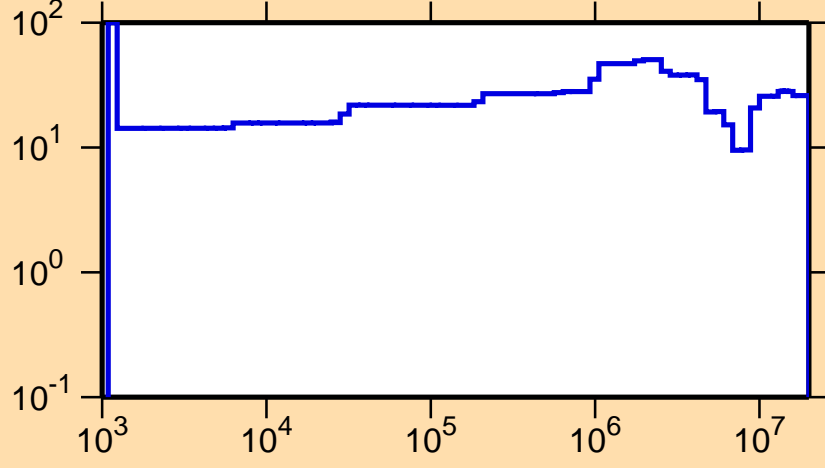
\Delta\sigma/\sigma vs. E for ^{207}\text{Po}(n,\gamma)
