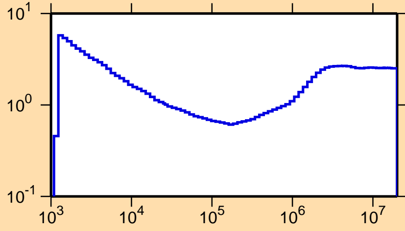
\sigma vs. E for ^{207}\text{Po}(n,\text{nonel.})
