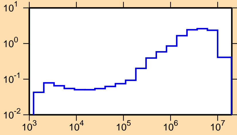
\sigma vs. E for ^{207}\text{Po}(n,\text{inel.})
