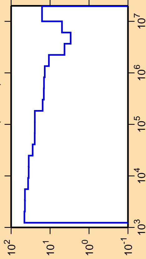
\Delta\sigma/\sigma vs. E for ^{207}\text{Po}(n,\text{inel.})
