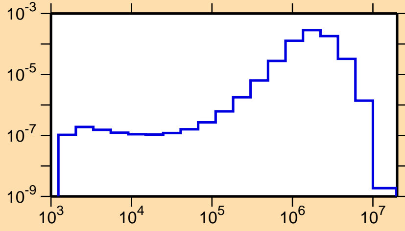
\sigma vs. E for ^{207}\text{Po}(n,n_2)
