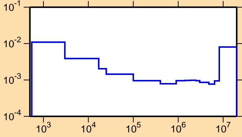
\sigma vs. E for ^{207}\text{Po}(n,\alpha)
