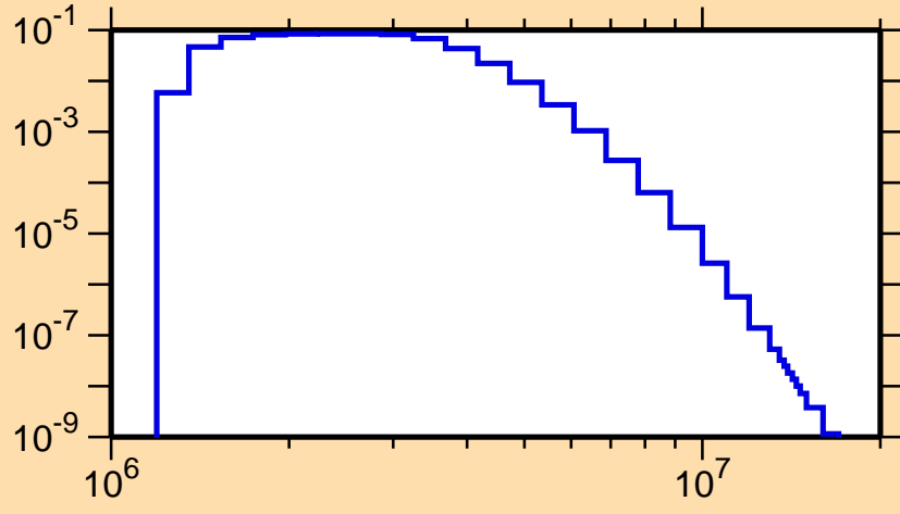
\sigma vs. E for ^{208}\text{Po}(n,n_3)
