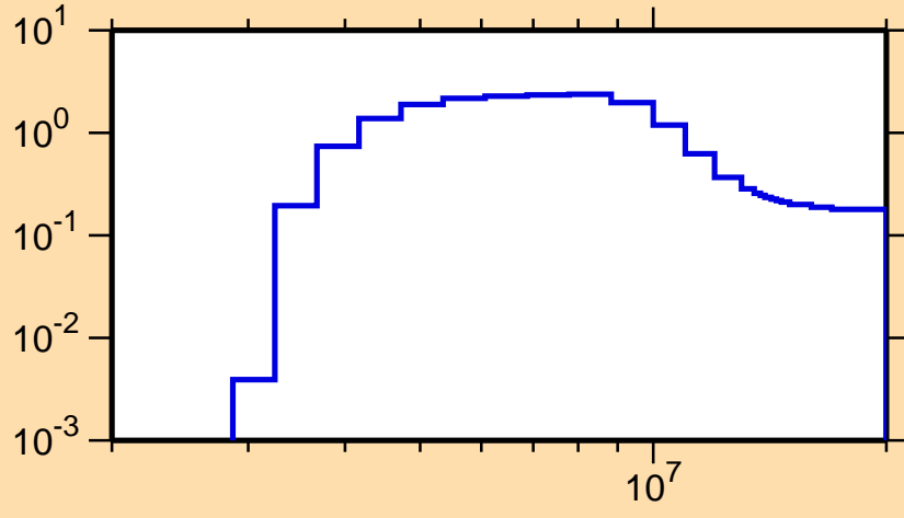
\sigma vs. E for ^{208}\text{Po}(n,n\text{cont.})
