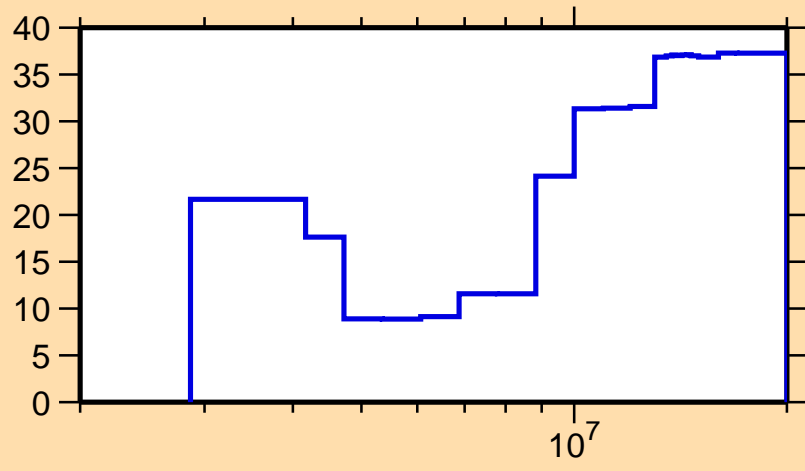
\Delta\sigma/\sigma vs. E for ^{208}\text{Po}(n,n\text{cont.})
