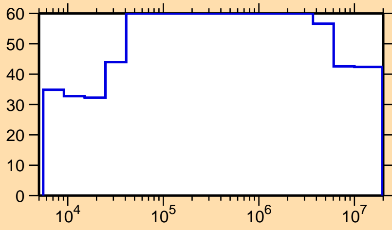
\Delta\sigma/\sigma vs. E for ^{208}\text{Po}(n,p)
