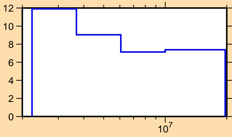
\Delta\sigma/\sigma vs. E for ^{208}\text{Po}(n,n\text{onel.})
