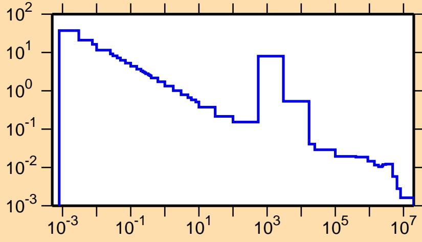
\sigma vs. E for ^{208}\text{Po}(n,\gamma)
