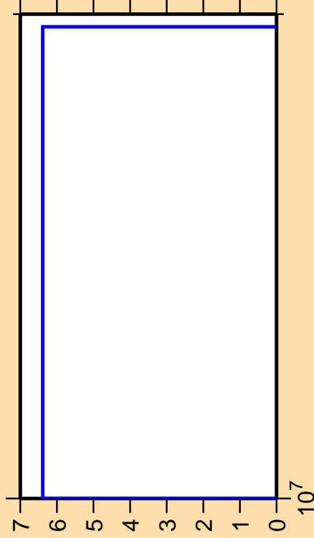
\Delta\sigma/\sigma vs. E for ^{209}\text{Po}(n,\text{pt})
