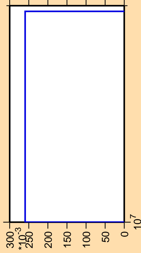
\Delta\sigma/\sigma vs. E for ^{209}\text{Po}(\text{mt } 34)
