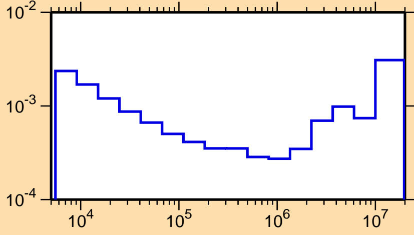
\sigma vs. E for ^{209}\text{Po}(n,\alpha)
