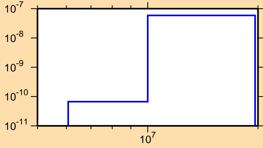
\sigma vs. E for ^{209}\text{Po}(n,p\alpha)
