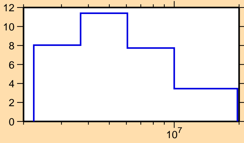
\Delta\sigma/\sigma vs. E for ^{209}\text{Po}(n, \text{tot.})
