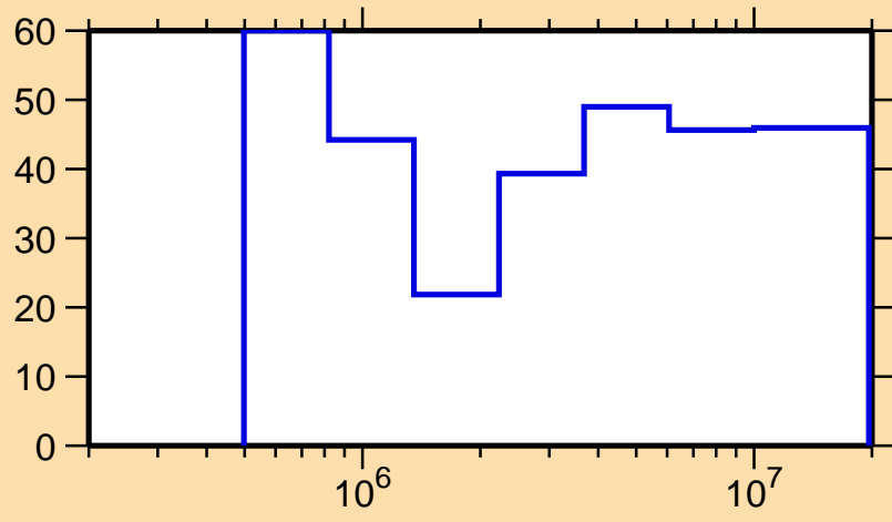
\Delta\sigma/\sigma vs. E for ^{209}\text{Po}(n,n_1)
