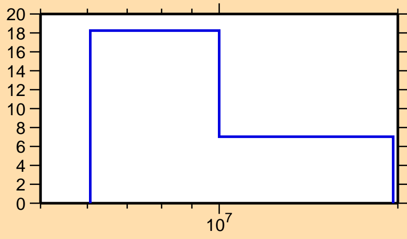
\Delta\sigma/\sigma vs. E for ^{209}\text{Po}(n,2n)
