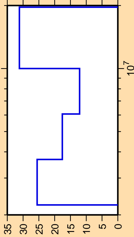
\Delta\sigma/\sigma vs. E for ^{209}\text{Po}(n,n\text{cont.})
