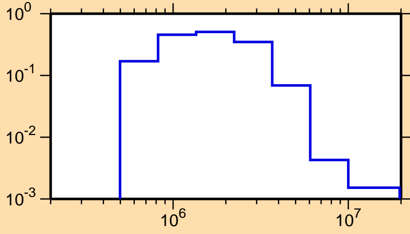
\sigma vs. E for ^{209}\text{Po}(n,n_1)
