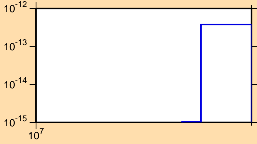
\sigma vs. E for ^{210}\text{Po} (mt 34)
