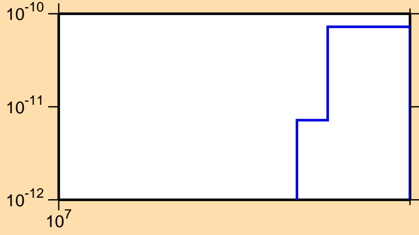
\sigma vs. E for ^{210}\text{Po} (mt 45)
