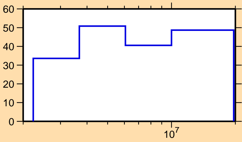
\Delta\sigma/\sigma vs. E for ^{210}\text{Po}(n,n_1)
