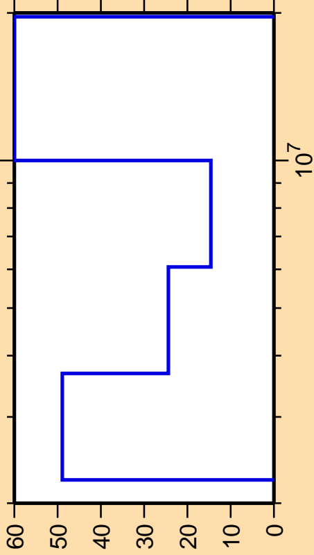
\Delta\sigma/\sigma vs. E for ^{210}\text{Po}(n,n_{\text{cont}}) .
