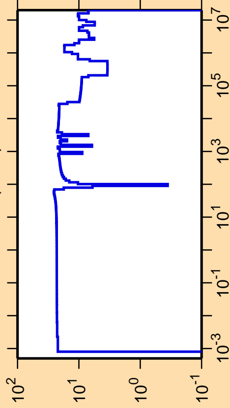
\Delta\sigma/\sigma vs. E for ^{211}\text{Po}(n,\text{el.})
