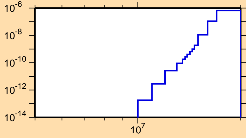
\sigma vs. E for ^{211}\text{Po}(\text{mt117})
