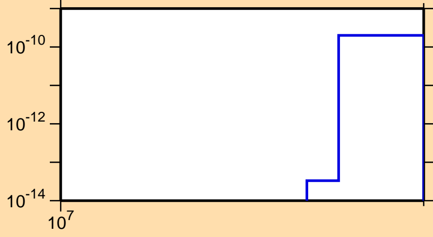
\sigma vs. E for ^{211}\text{Po} (mt 11)
