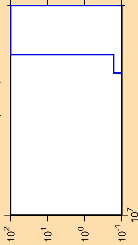
\Delta\sigma/\sigma vs. E for ^{211}\text{Po} (mt 11)
