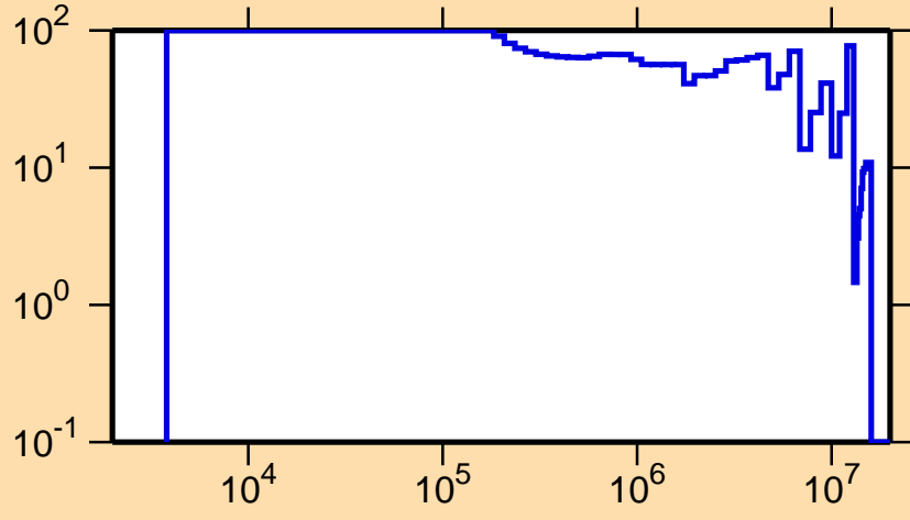
\Delta\sigma/\sigma vs. E for ^{211}\text{Po}(n,n_1)
