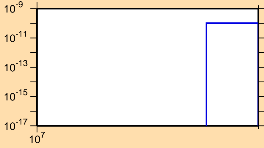
\sigma vs. E for ^{211}\text{Po} (mt 42)
