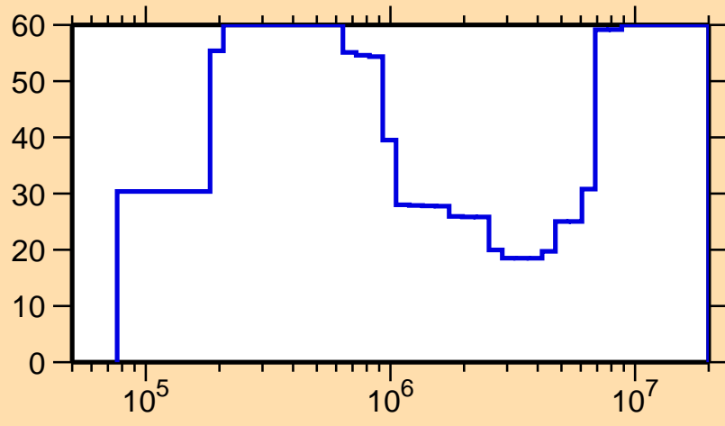
\Delta\sigma/\sigma vs. E for ^{211}\text{Po}(n,n\text{cont.})
