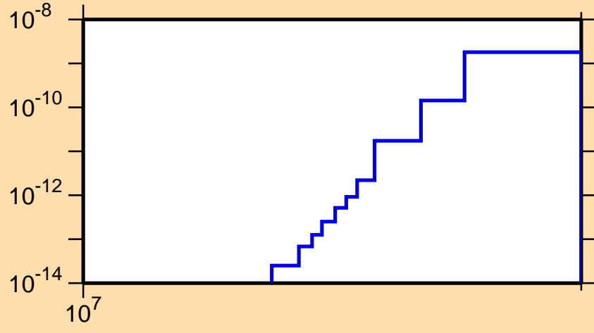
\sigma vs. E for ^{211}\text{Po}(\text{mt } 34)
