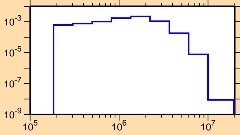
\sigma vs. E for ^{211}\text{Po}(n,n_2)
