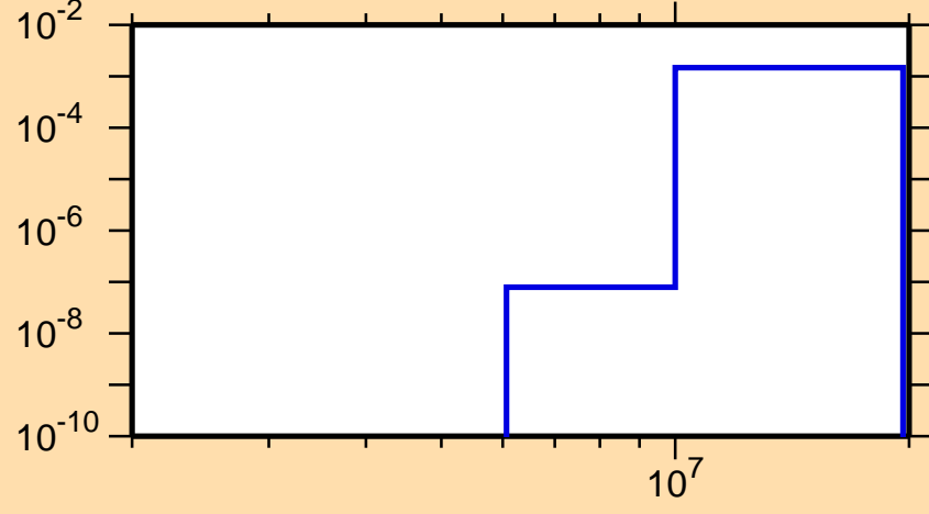
\sigma vs. E for ^{211}\text{Po}(n,t)
