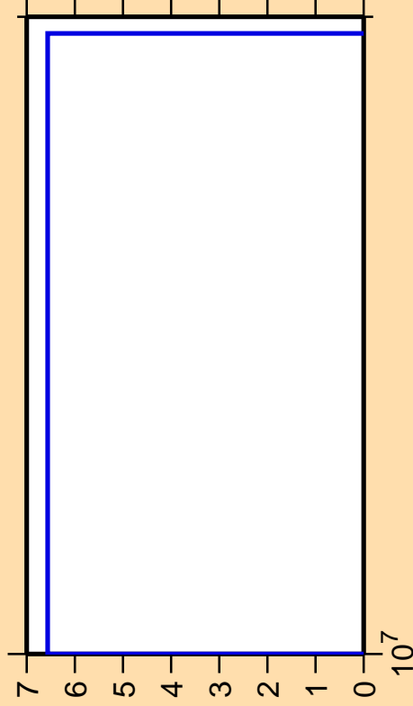
\Delta\sigma/\sigma vs. E for ^{211}\text{Po} (mt 11)
