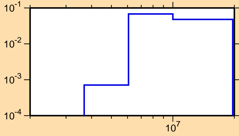
\sigma vs. E for ^{211}\text{Po}(n,2n\alpha)
