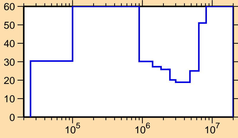
\Delta\sigma/\sigma vs. E for ^{211}\text{Po}(n,n\text{cont.})
