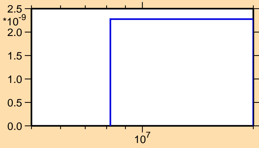
\sigma vs. E for ^{211}\text{Po}(\text{mt } 45)
