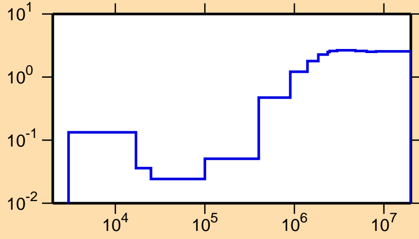
\sigma vs. E for ^{211}\text{Po}(n,\text{nonel.})
