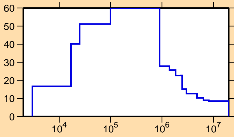
\Delta\sigma/\sigma vs. E for ^{211}\text{Po}(n,\text{nonel.})
