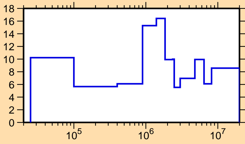
\Delta\sigma/\sigma vs. E for ^{211}\text{Po}(n, el.)
