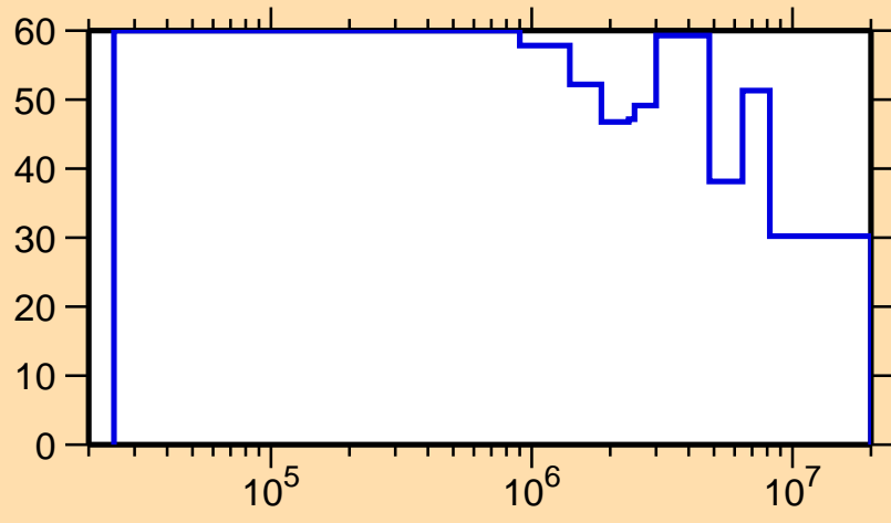
\Delta\sigma/\sigma vs. E for ^{211}\text{Po}(n,n_1)
