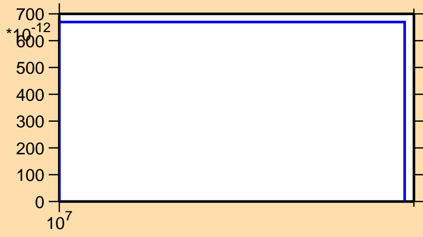
\sigma vs. E for ^{212}\text{Po} (mt 11)
