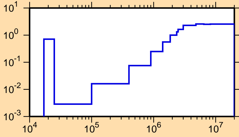
\sigma vs. E for ^{212}\text{Po}(n,\text{nonel.})
