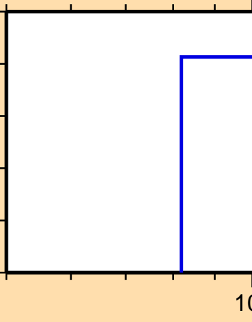
\sigma vs. E for ^{212}\text{Po}(n,\text{He}3)
