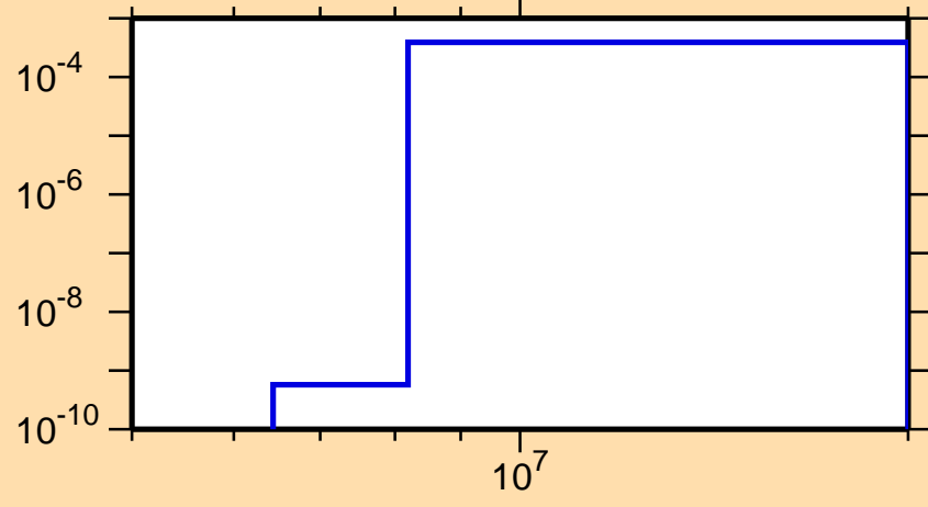
\sigma vs. E for ^{212}\text{Po}(\text{mt } 45)
