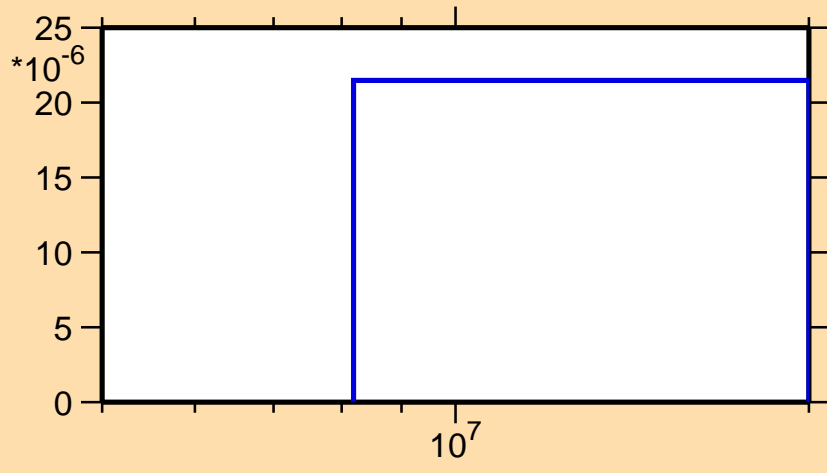
\sigma vs. E for ^{212}\text{Po}(n,\text{nd})
