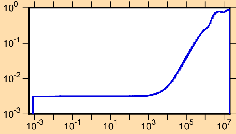
\mu vs. E for ^{217}\text{Po}(\text{mt251})
