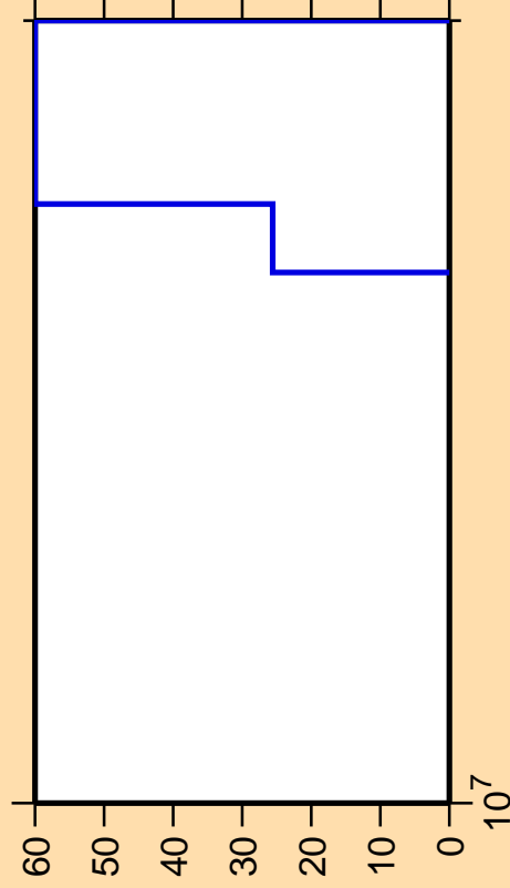
\Delta\sigma/\sigma vs. E for ^{217}\text{Po}(\text{mt117})
