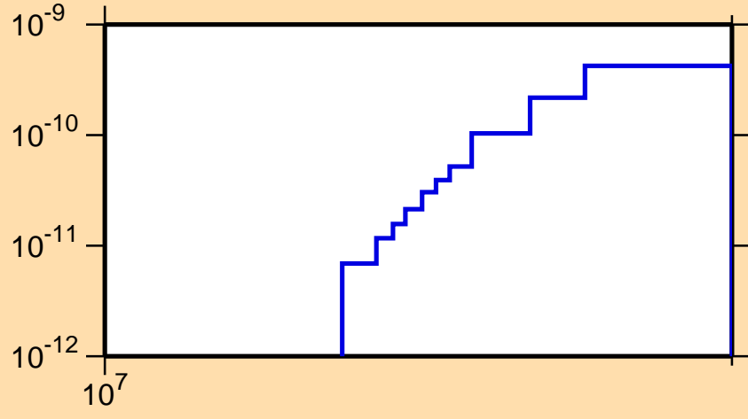
\sigma vs. E for ^{217}\text{Po}(n,p\alpha)
