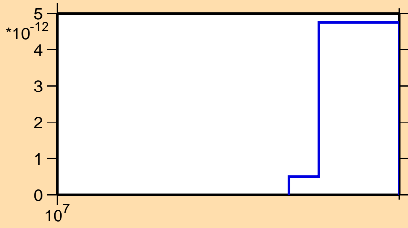
\sigma vs. E for ^{217}\text{Po} (mt 45)
