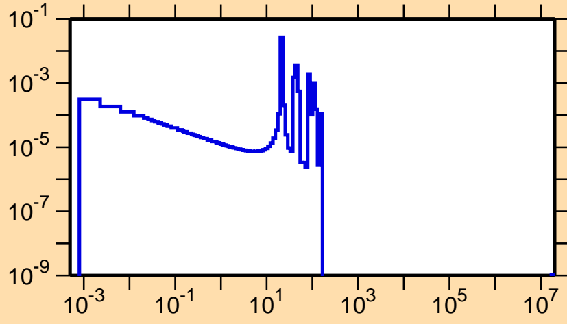
\sigma vs. E for ^{217}\text{Po}(n,f)
