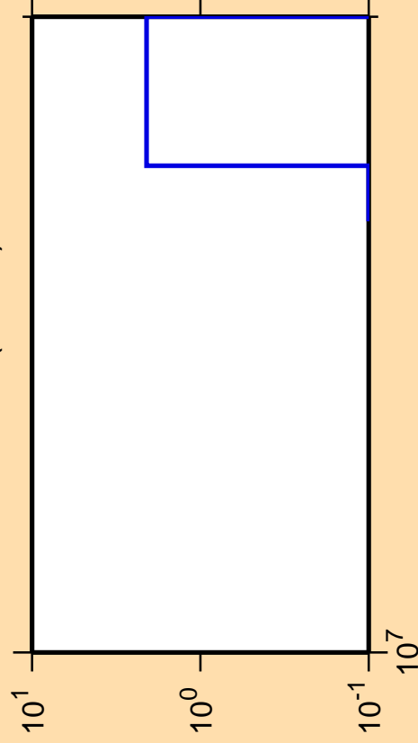
\Delta\sigma/\sigma vs. E for ^{217}\text{Po} (mt 42)
