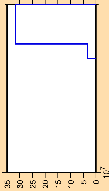
\Delta\sigma/\sigma vs. E for ^{217}\text{Po} (mt 45)
