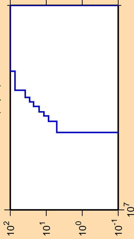
\Delta\sigma/\sigma vs. E for ^{217}\text{Po}(n,p\alpha)
