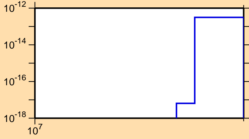
\sigma vs. E for ^{217}\text{Po} (mt 42)
