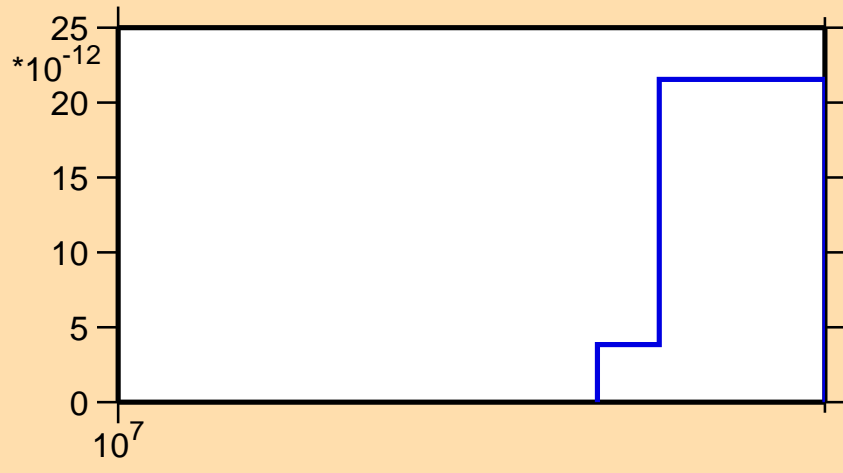
\sigma vs. E for ^{217}\text{Po}(\text{mt117})
