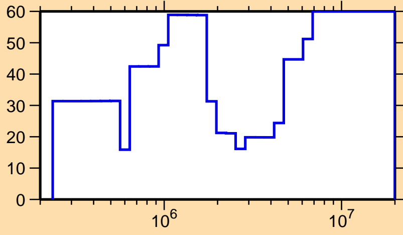
\Delta\sigma/\sigma vs. E for ^{217}\text{Po}(n,\text{el.})
