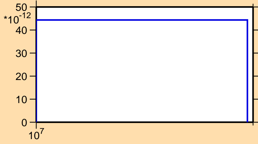
\sigma vs. E for ^{217}\text{Po}(n,p\alpha)
