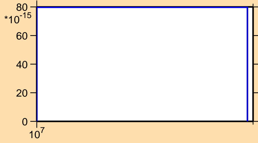
\sigma vs. E for ^{217}\text{Po}(\text{mt } 45)
