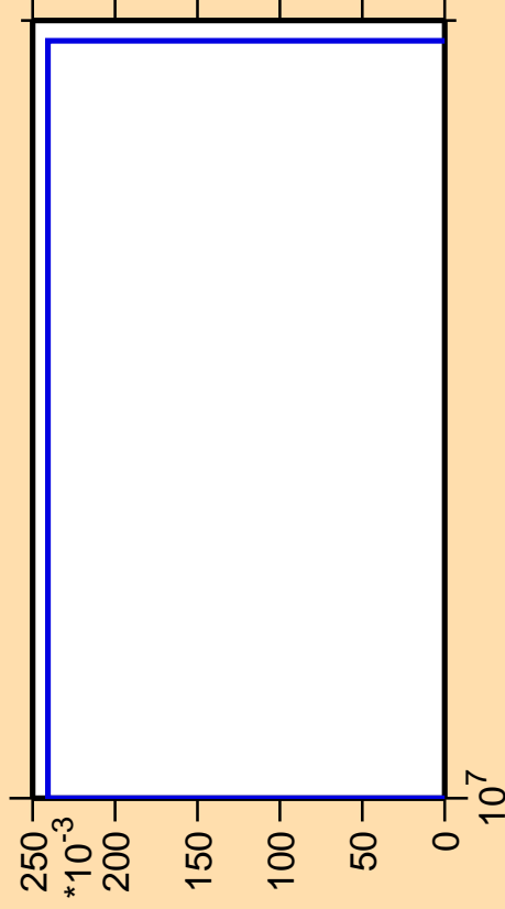
\Delta\sigma/\sigma vs. E for ^{217}\text{Po} (mt 11)
