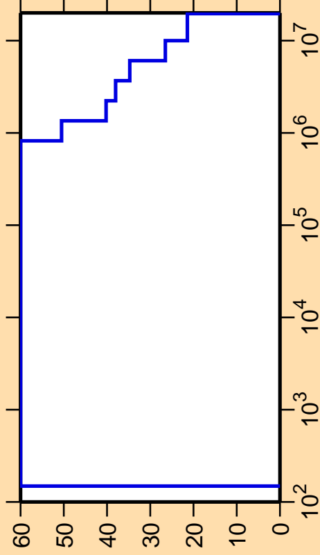
\Delta\sigma/\sigma vs. E for ^{217}\text{Po}(n,\text{nonel.})
