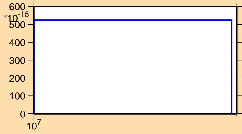
\sigma vs. E for ^{217}\text{Po}(\text{mt117})
