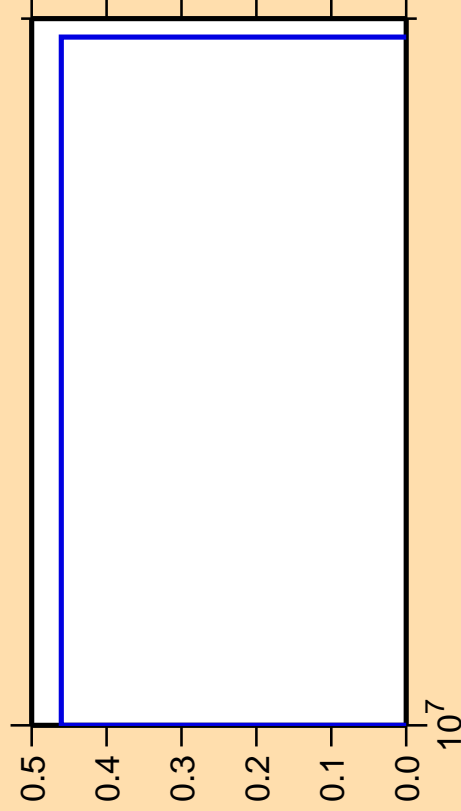
\Delta\sigma/\sigma vs. E for ^{217}\text{Po}(\text{mt } 45)
