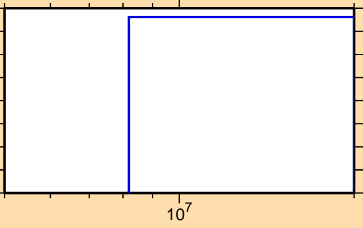
\sigma vs. E for ^{217}\text{Po}(n,nt)
