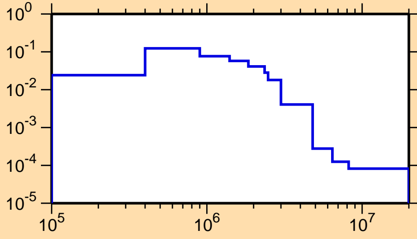
\sigma vs. E for ^{217}\text{Po}(n,n_1)
