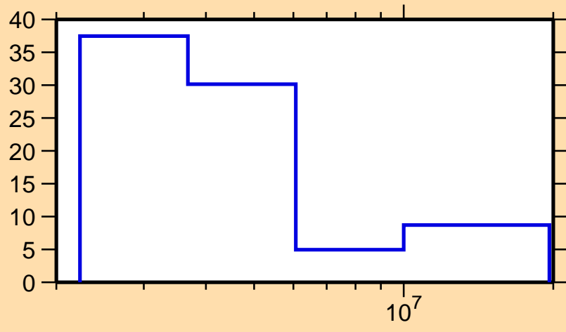
\Delta\sigma/\sigma vs. E for ^{218}\text{Po}(n,\text{tot.})
