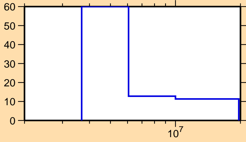
\Delta\sigma/\sigma vs. E for ^{218}\text{Po}(n,2n)
