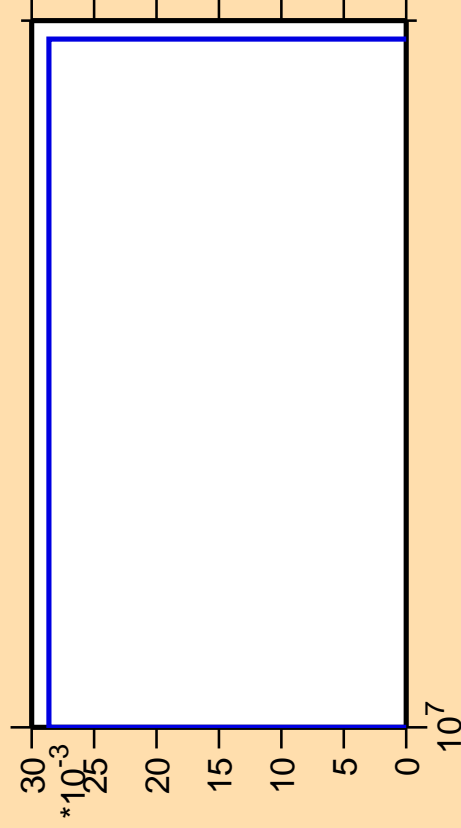
\Delta\sigma/\sigma vs. E for ^{218}\text{Po}(\text{mt 11})
