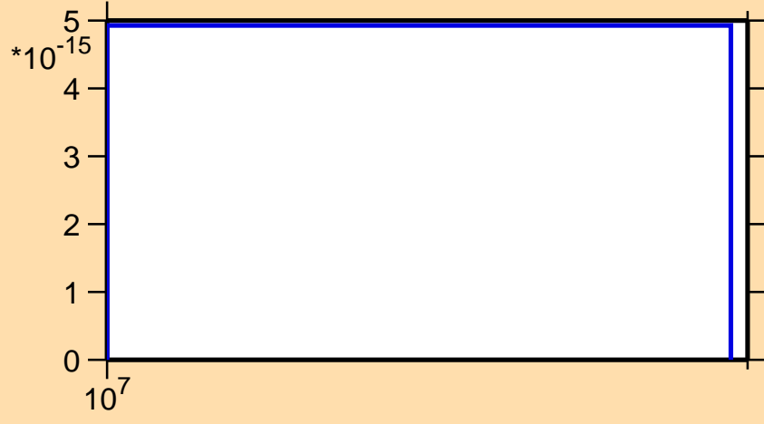
\sigma vs. E for ^{218}\text{Po} (mt 45)
