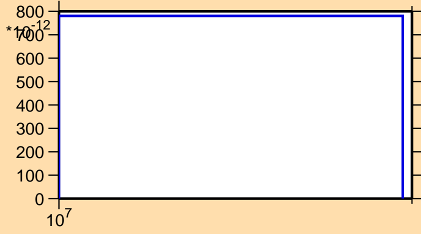
\sigma vs. E for ^{218}\text{Po}(n,2np)
