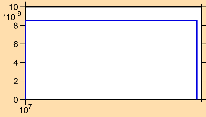
\sigma vs. E for ^{218}\text{Po}(n,\text{nd})
