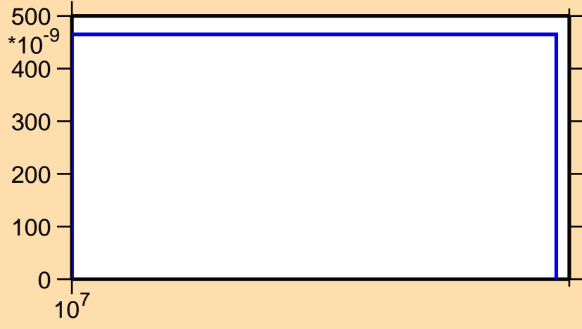
\sigma vs. E for ^{218}\text{Po}(n,nt)
