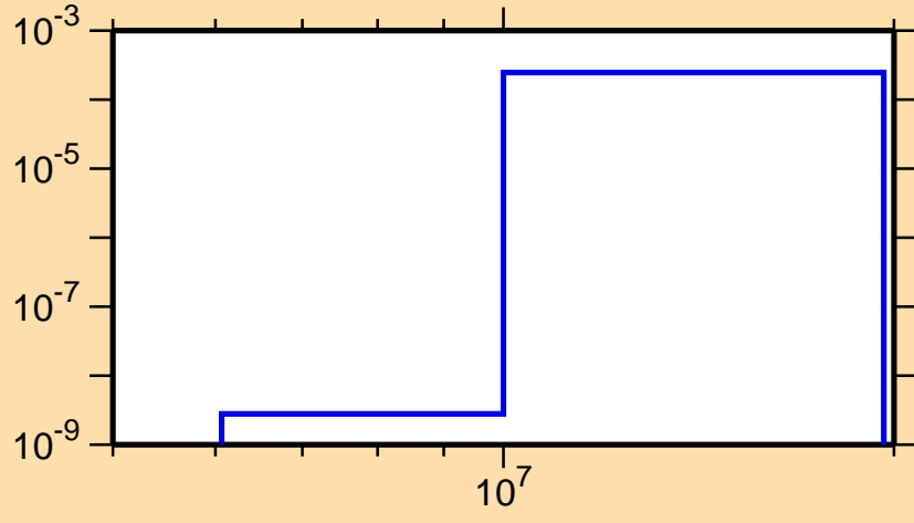
\sigma vs. E for ^{218}\text{Po}(n,p)
