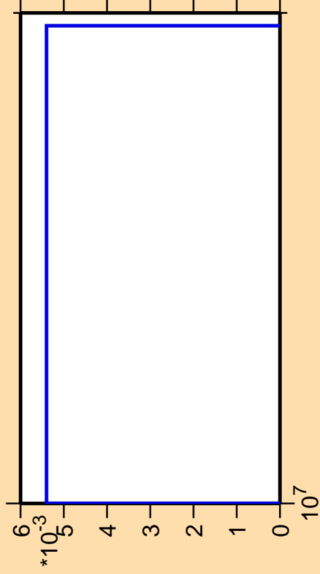
\Delta\sigma/\sigma vs. E for ^{218}\text{Po}(n,\text{He}3)
