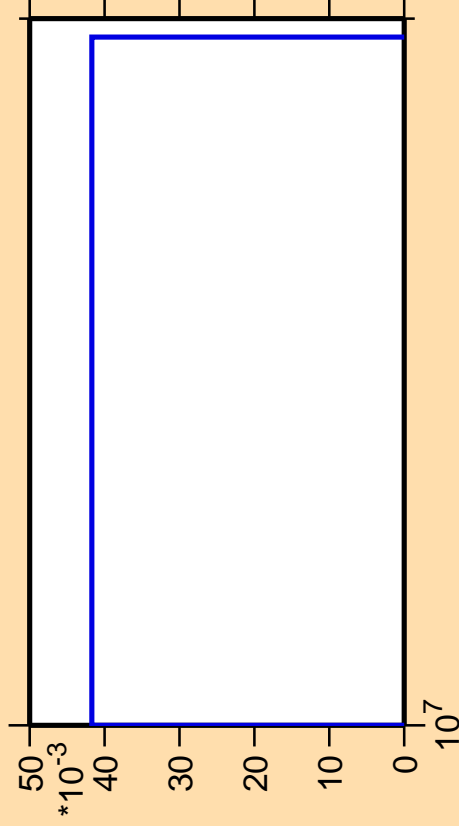
\Delta\sigma/\sigma vs. E for ^{218}\text{Po} (mt 45)
