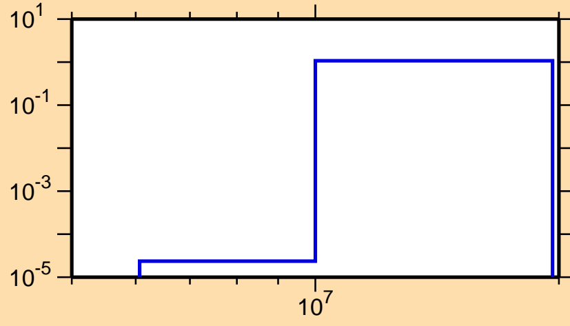
\sigma vs. E for ^{218}\text{Po}(n,3n)
