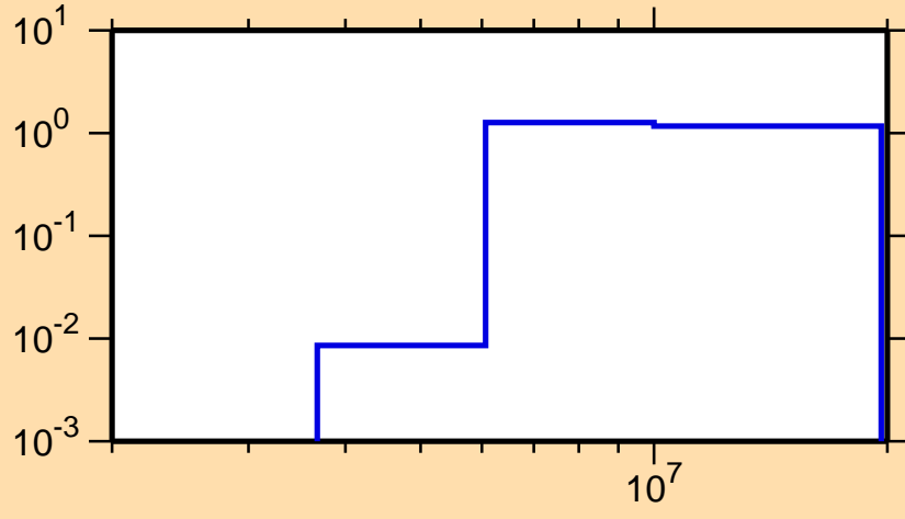
\sigma vs. E for ^{218}\text{Po}(n,2n)
