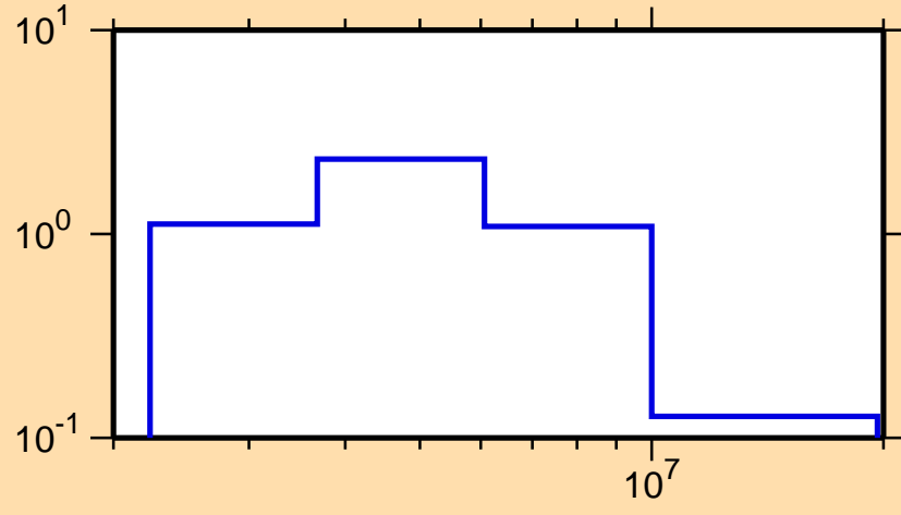
\sigma vs. E for ^{218}\text{Po}(n,n\text{cont.})
