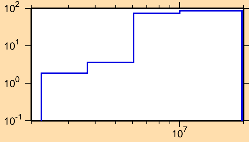
\Delta\sigma/\sigma vs. E for ^{218}\text{Po}(n, n_1)
