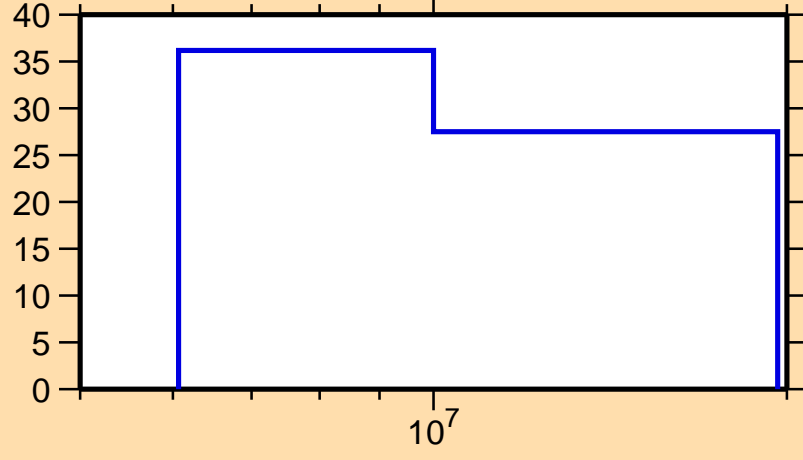
\Delta\sigma/\sigma vs. E for ^{218}\text{Po}(n,p)
