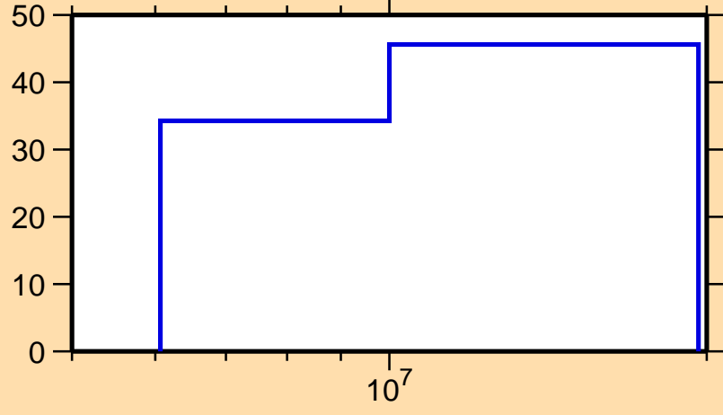
\Delta\sigma/\sigma vs. E for ^{218}\text{Po}(n,n\text{cont.})
