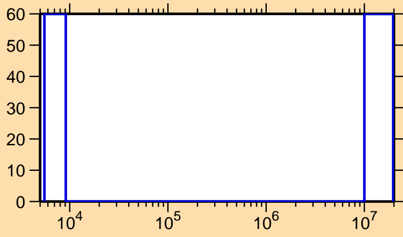
\Delta\sigma/\sigma vs. E for ^{218}\text{Po}(n,f)
