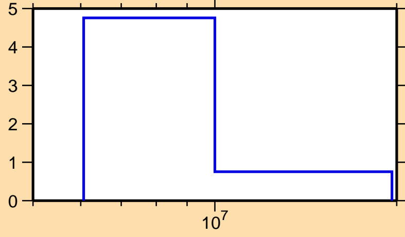
\Delta\sigma/\sigma vs. E for ^{218}\text{Po}(n,\text{nonel.})
