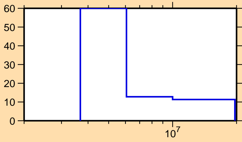
\Delta\sigma/\sigma vs. E for ^{218}\text{Po}(n,2n)
