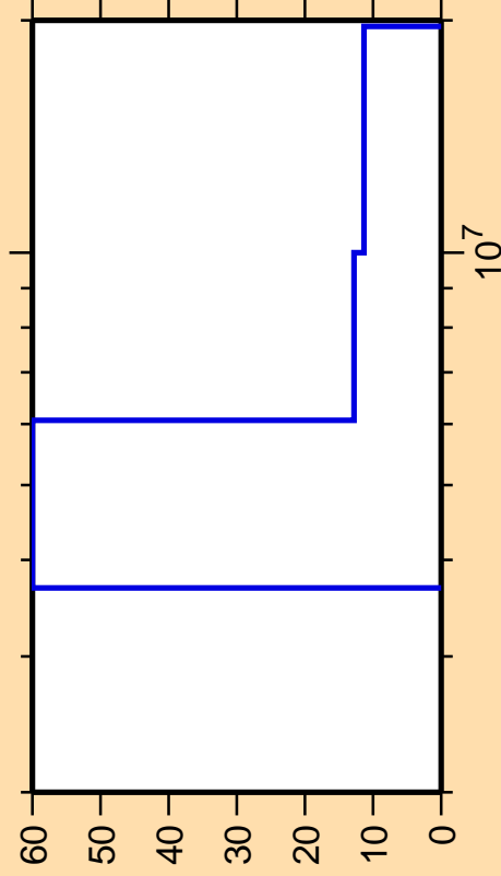
\Delta\sigma/\sigma vs. E for ^{218}\text{Po}(n,2n)
