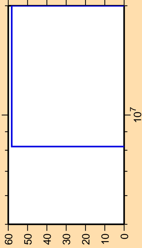
\Delta\sigma/\sigma vs. E for ^{218}\text{Po}(n,np)
