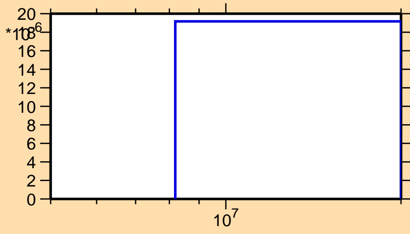
\sigma vs. E for ^{218}\text{Po}(n,np)
