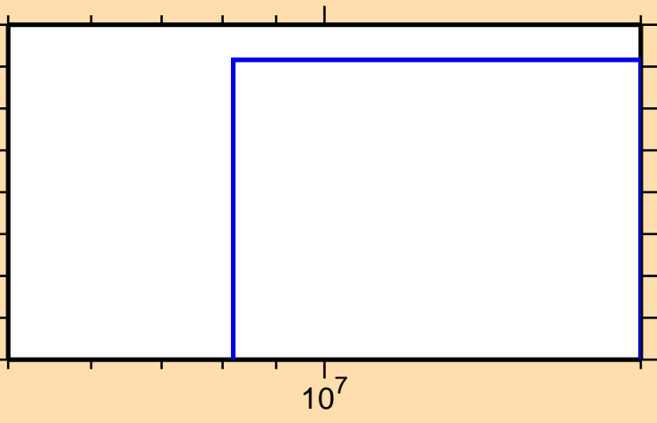
\sigma vs. E for ^{218}\text{Po}(n,3n\alpha)
