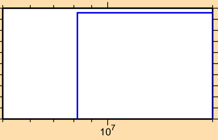
\sigma vs. E for ^{218}\text{Po}(n,np)
