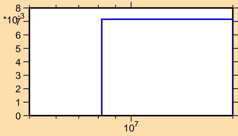
\sigma vs. E for ^{218}\text{Po}(n,3n\alpha)
