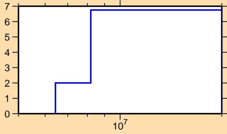
\Delta\sigma/\sigma vs. E for ^{218}\text{Po}(n,\text{tot.})
