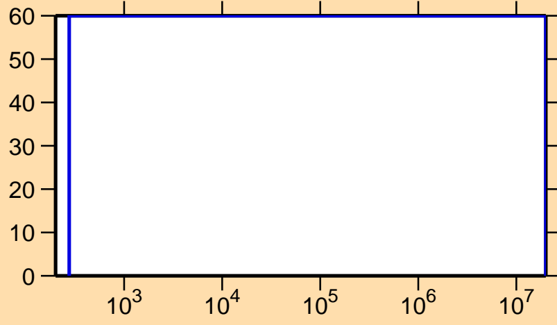
\Delta\sigma/\sigma vs. E for ^{219}\text{Po}(n,\gamma)
