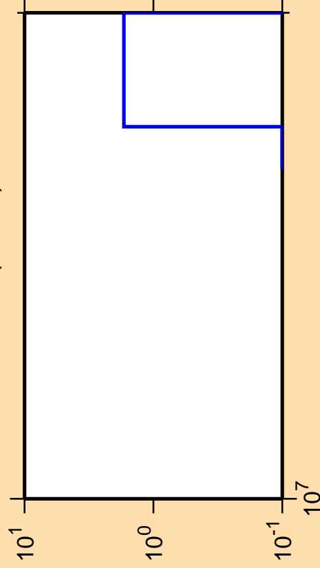
\Delta\sigma/\sigma vs. E for ^{219}\text{Po} (mt 42)
