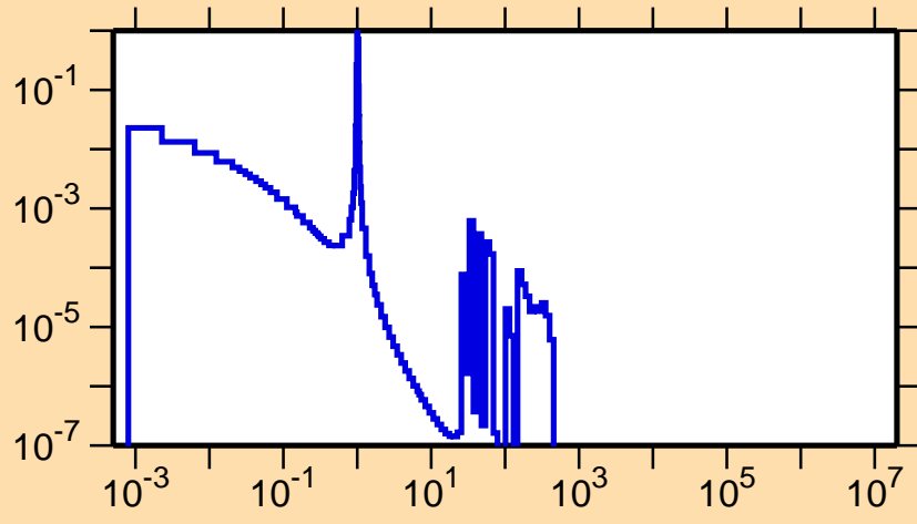
\sigma vs. E for ^{219}\text{Po}(n,f)
