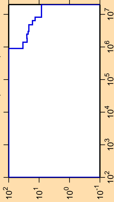
\Delta\sigma/\sigma vs. E for ^{219}\text{Po}(n,\text{nonel.})
