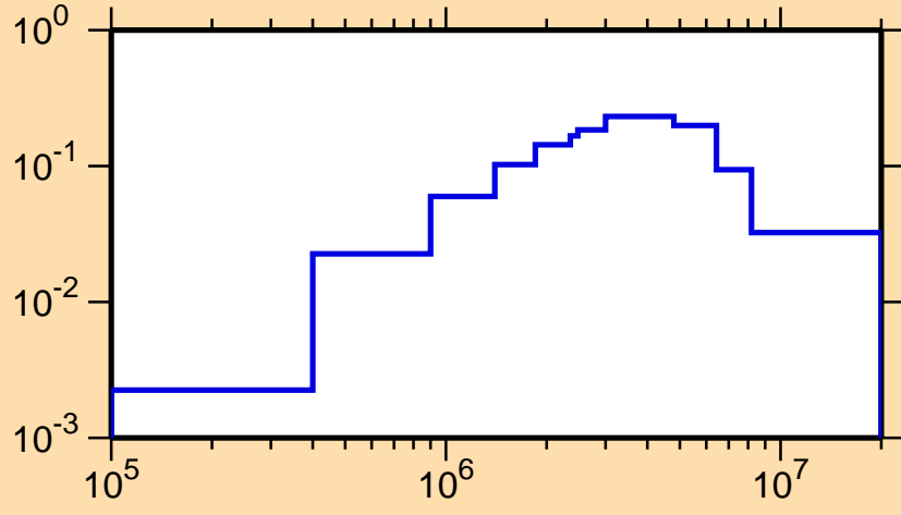
\sigma vs. E for ^{219}\text{Po}(n,n\alpha)
