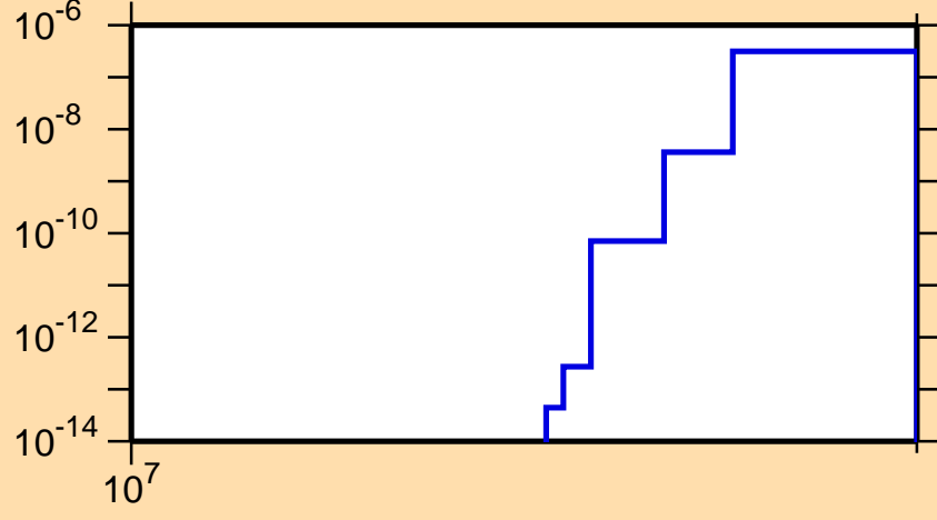
\sigma vs. E for ^{220}\text{Po}(n,\text{nd})
