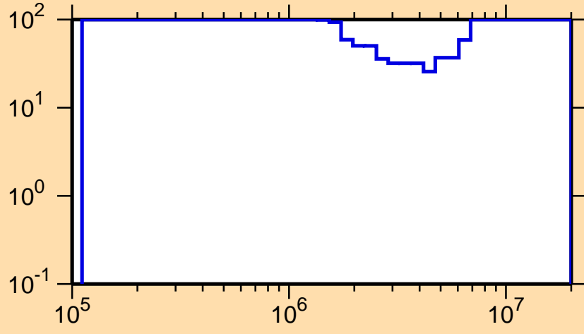
\Delta\sigma/\sigma vs. E for ^{220}\text{Po}(n,n\text{cont.})
