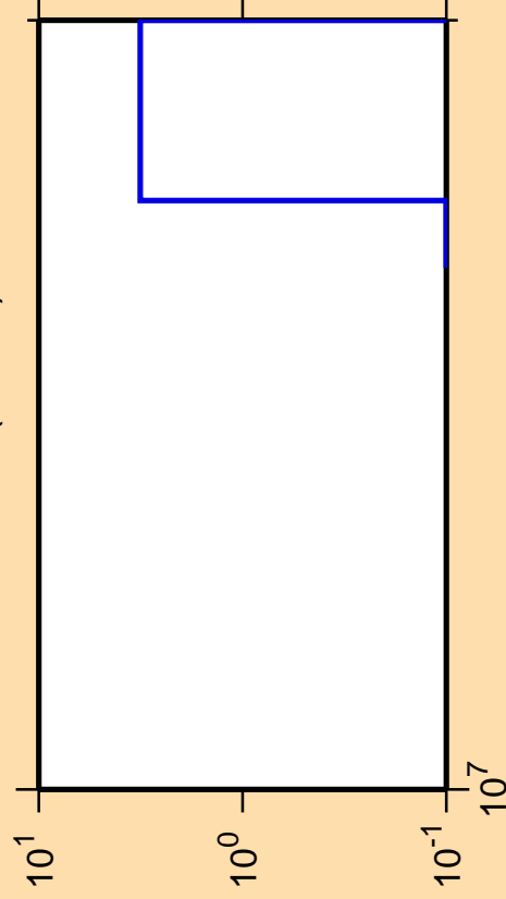
\Delta\sigma/\sigma vs. E for ^{220}\text{Po}(\text{mt 11})
