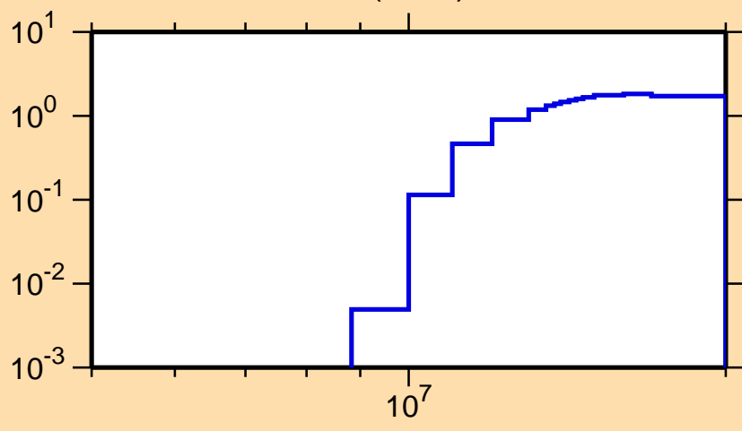
\sigma vs. E for ^{220}\text{Po}(n,3n)
