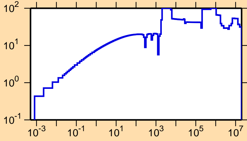
\Delta\sigma/\sigma vs. E for ^{220}\text{Po}(n,\text{tot.})
