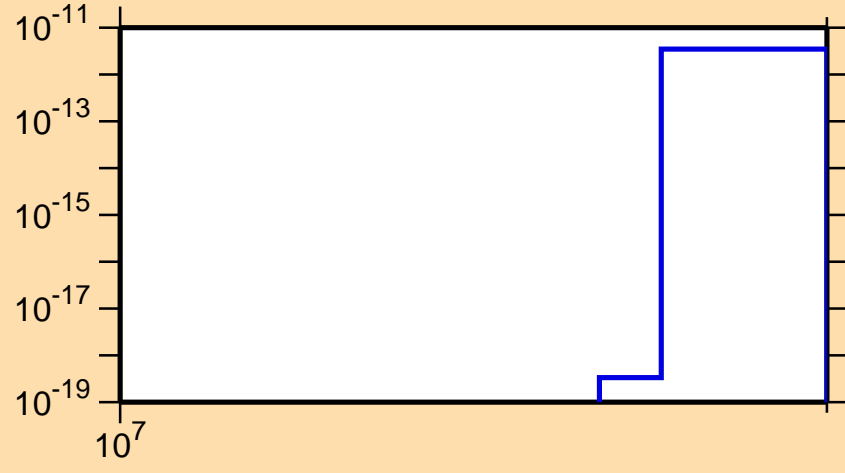
\sigma vs. E for ^{220}\text{Po}(\text{mt 11})
