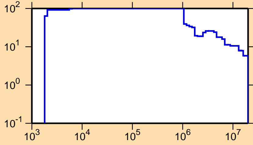
\Delta\sigma/\sigma vs. E for ^{220}\text{Po}(n,\text{nonel.})
