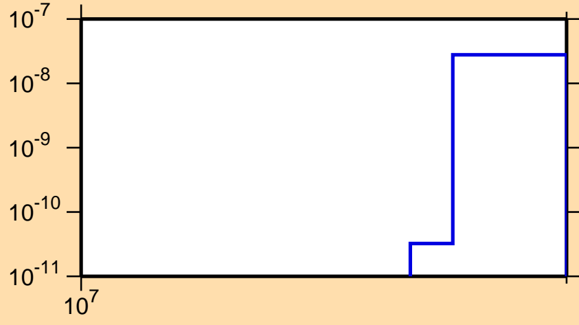
\sigma vs. E for ^{220}\text{Po}(n,2np)
