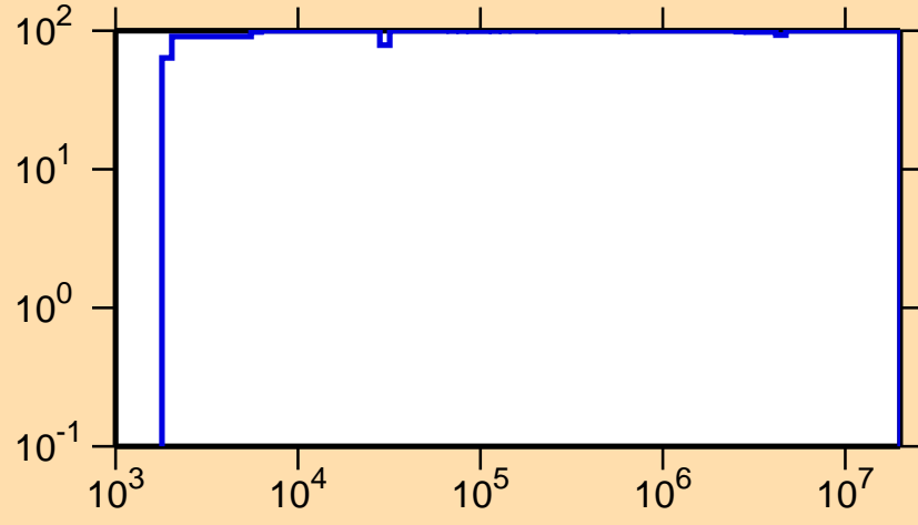
\Delta\sigma/\sigma vs. E for ^{220}\text{Po}(n,\gamma)
