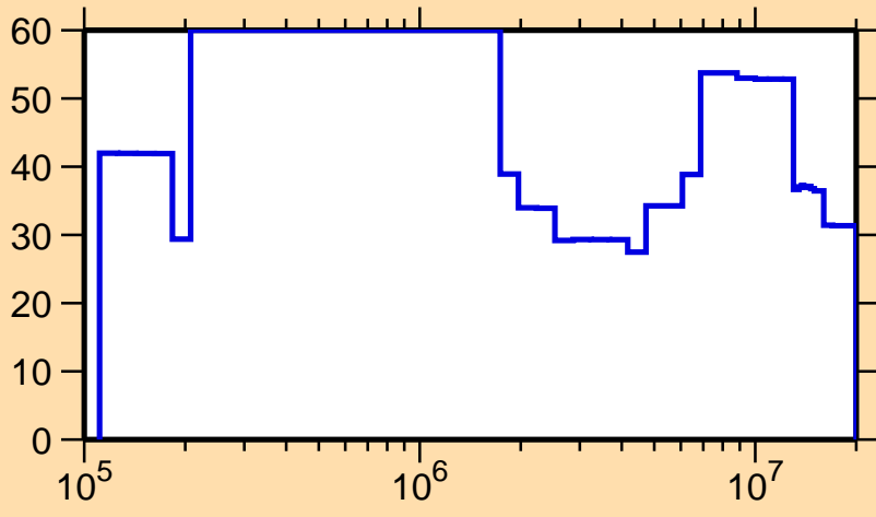
\Delta\sigma/\sigma vs. E for ^{220}\text{Po}(n,\text{tot.})
