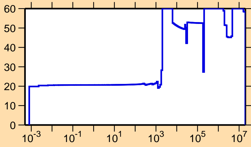
\Delta\sigma/\sigma vs. E for ^{220}\text{Po}(n,el.)
