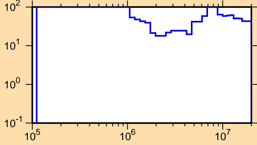
\Delta\sigma/\sigma vs. E for ^{220}\text{Po}(n,\text{inel.})
