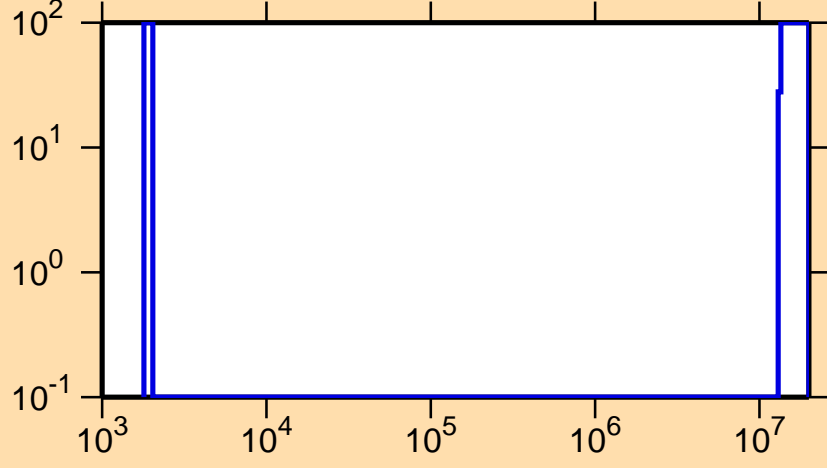
\Delta\sigma/\sigma vs. E for ^{220}\text{Po}(n,f)
