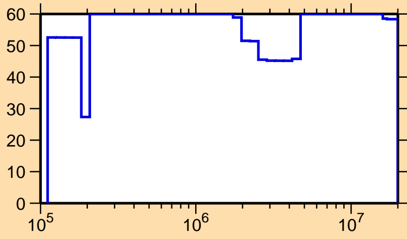
\Delta\sigma/\sigma vs. E for ^{220}\text{Po}(n,\text{el.})
