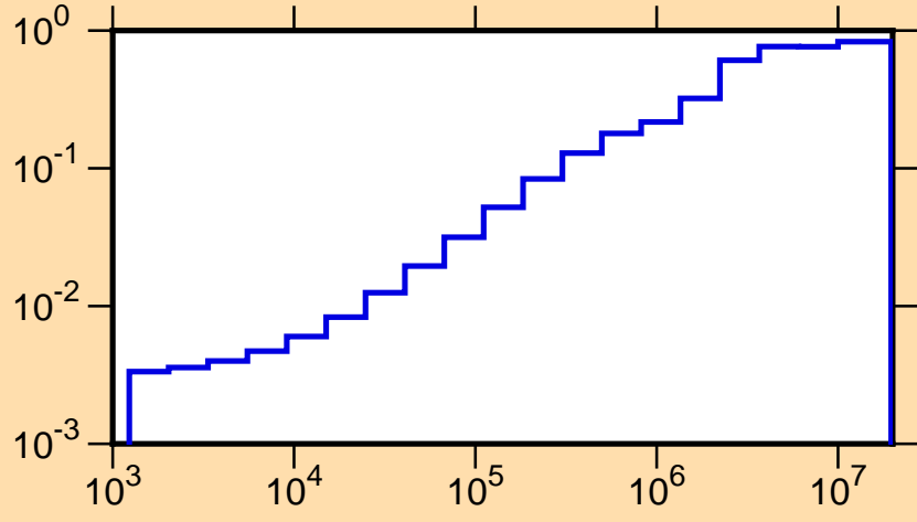
\mu vs. E for ^{220}\text{Po} (mt251)
