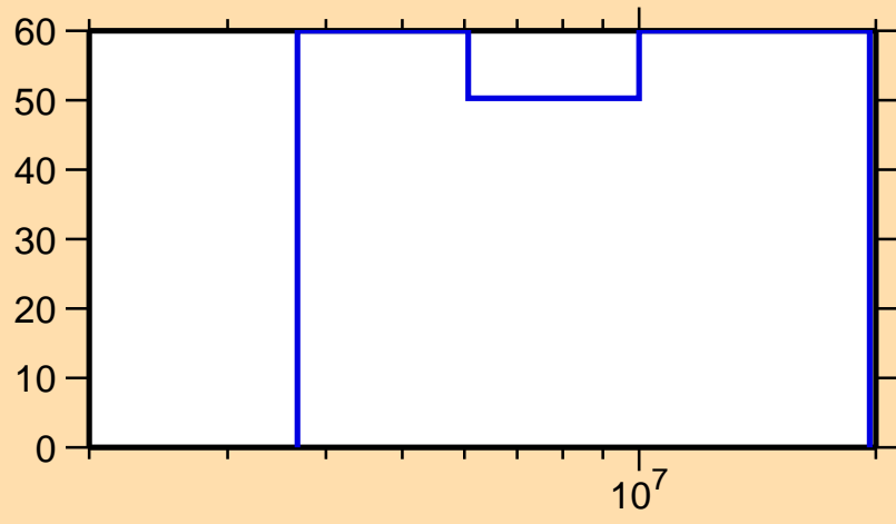
\Delta\sigma/\sigma vs. E for ^{220}\text{Po}(n,2n)
