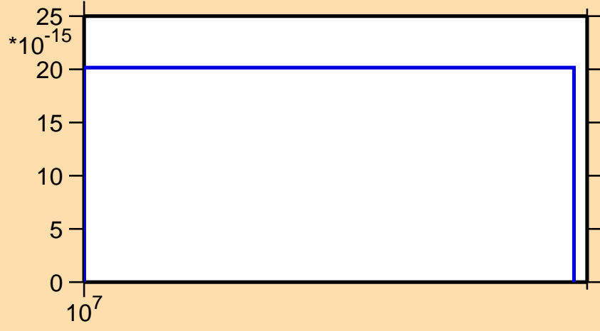
\sigma vs. E for ^{220}\text{Po} (mt 11)
