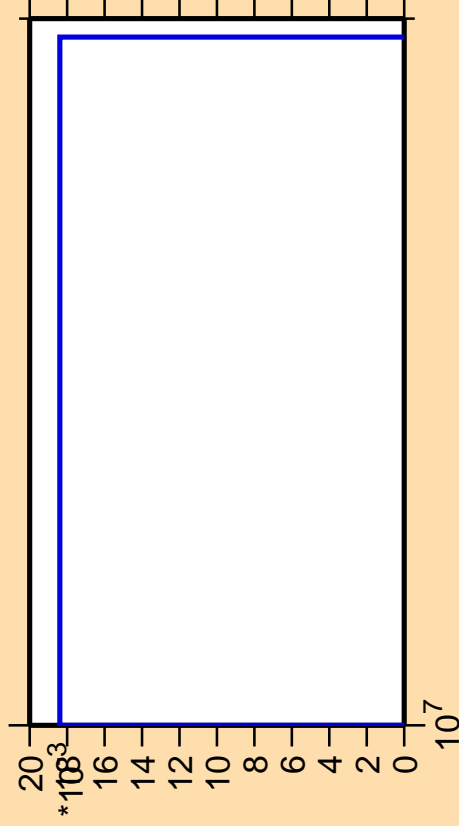
\Delta\sigma/\sigma vs. E for ^{220}\text{Po} (mt 11)
