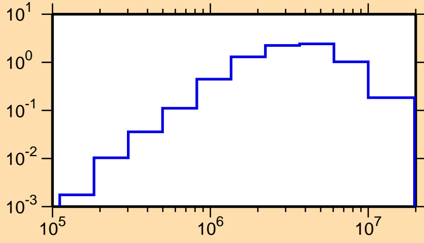
\sigma vs. E for ^{220}\text{Po}(n,n\text{cont.})
