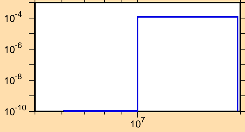
\sigma vs. E for ^{220}\text{Po}(n,p)
