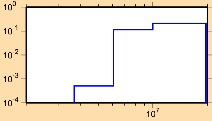
\sigma vs. E for ^{220}\text{Po}(n,2n\alpha)
