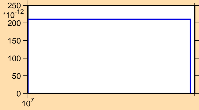
\sigma vs. E for ^{220}\text{Po}(n,2np)
