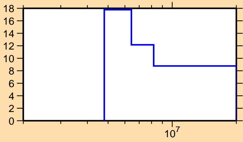
\Delta\sigma/\sigma vs. E for ^{220}\text{Po}(n,\text{nonel.})
