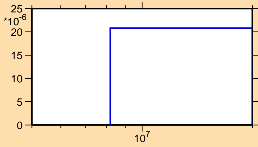
\sigma vs. E for ^{220}\text{Po}(n,t)
