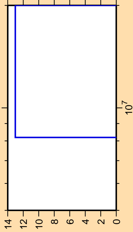
\Delta\sigma/\sigma vs. E for ^{220}\text{Po}(n,d)
