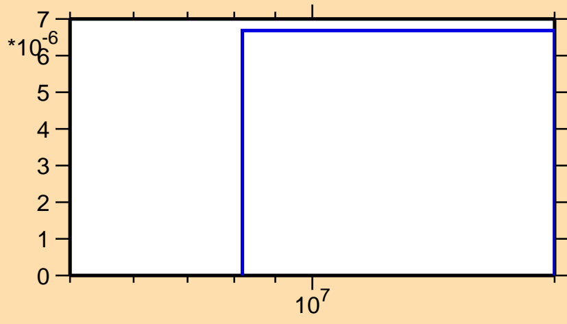
\sigma vs. E for ^{220}\text{Po}(n,np)
