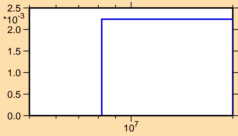
\sigma vs. E for ^{220}\text{Po}(n,3n\alpha)
