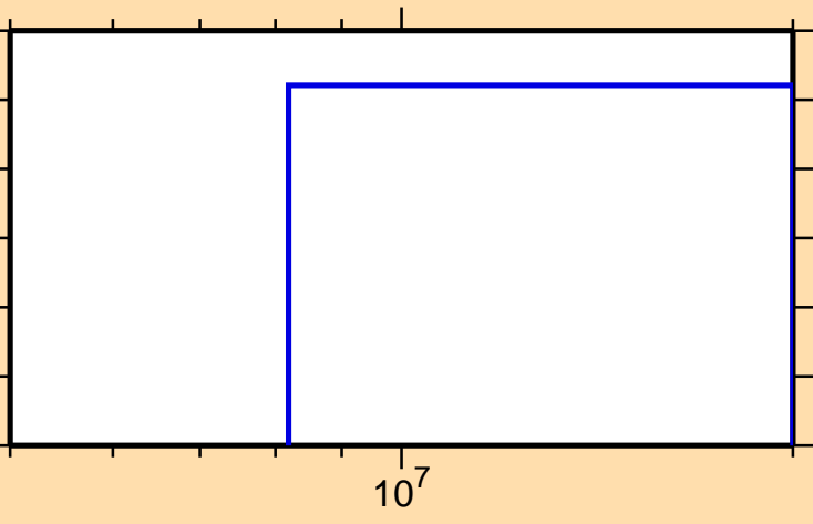
\sigma vs. E for ^{220}\text{Po}(n,d)
