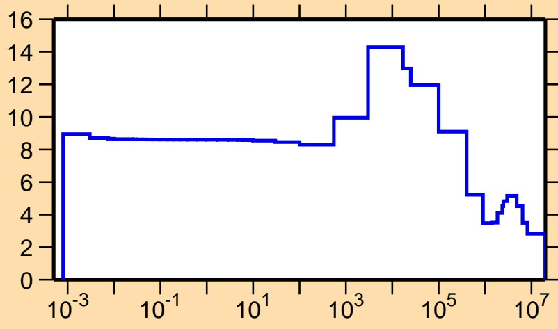
\sigma vs. E for ^{220}\text{Po}(n,\text{el.})
