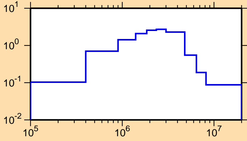
\sigma vs. E for ^{221}\text{Po}(n,\text{inel.})
