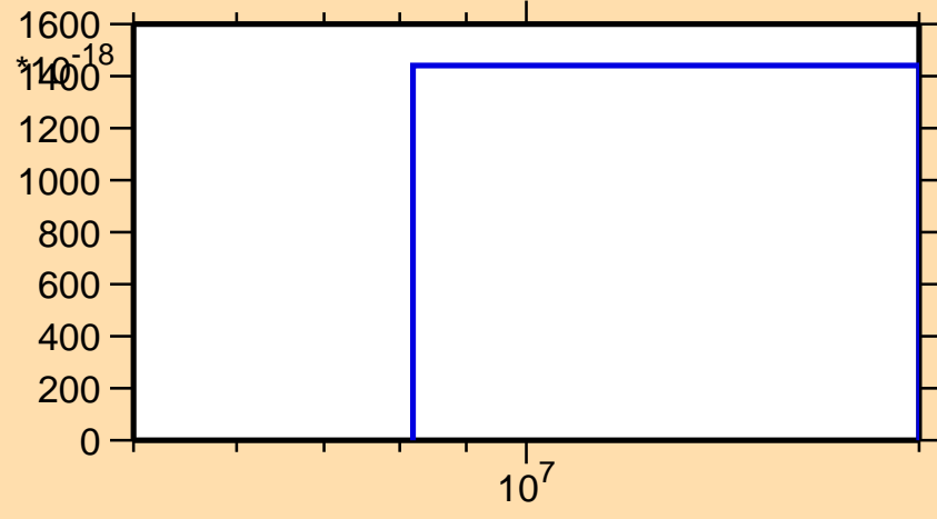
\sigma vs. E for ^{221}\text{Po}(n,\text{He}3)
