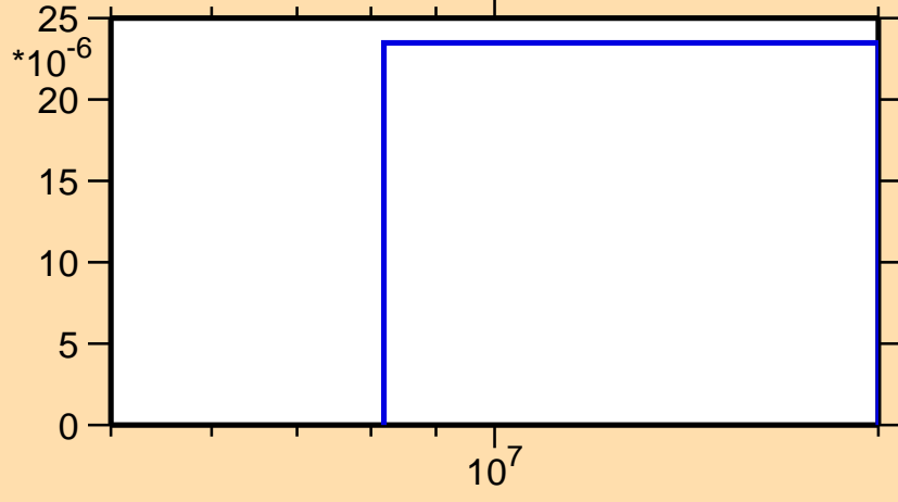
\sigma vs. E for ^{221}\text{Po}(n,d)
