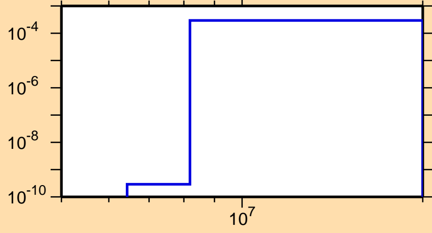
\sigma vs. E for ^{221}\text{Po}(n,p)
