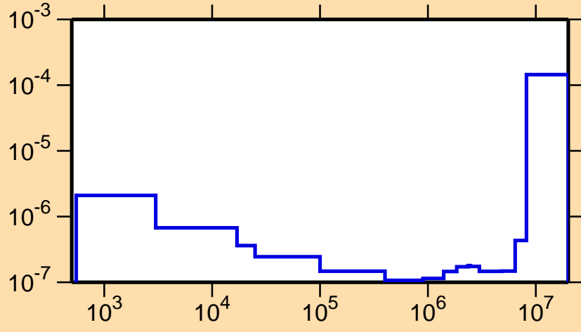
\sigma vs. E for ^{221}\text{Po}(n,\alpha)
