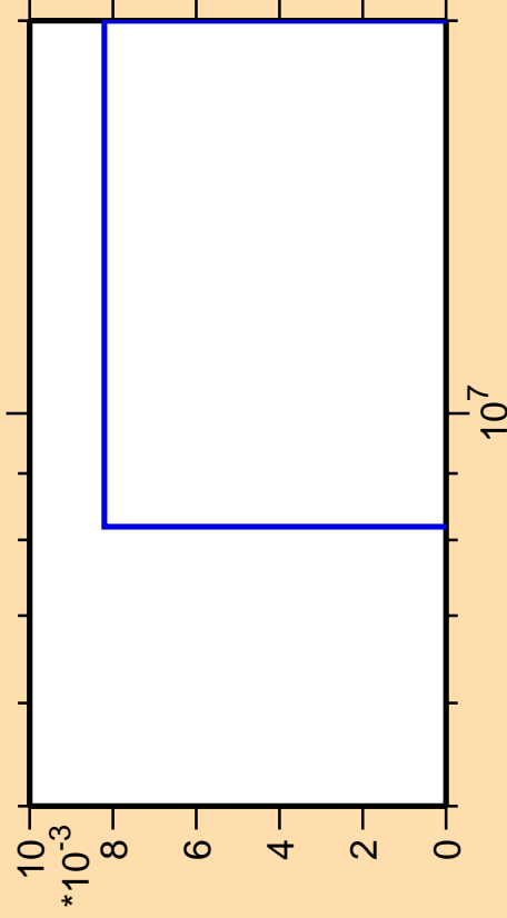
\Delta\sigma/\sigma vs. E for ^{221}\text{Po}(n,\text{He}3)
