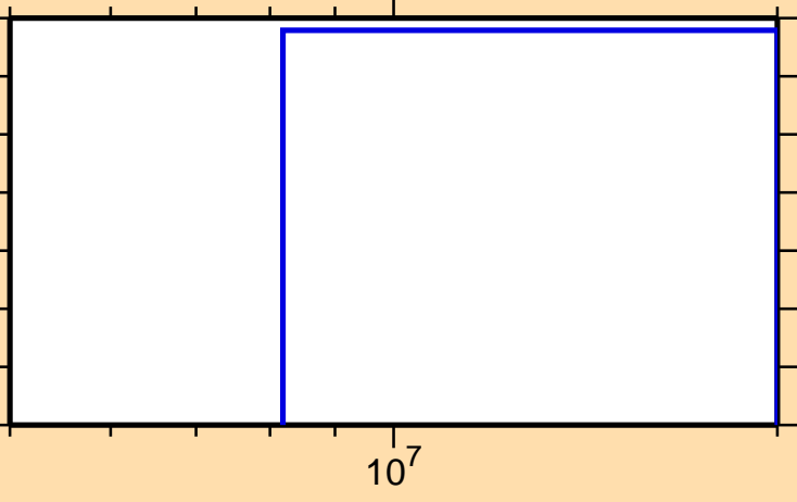
\sigma vs. E for ^{221}\text{Po}(n,\text{nd})
