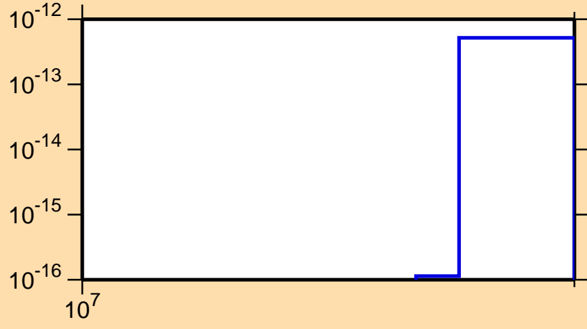
\sigma vs. E for ^{222}\text{Po} (mt 11)
