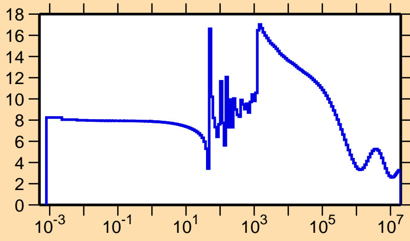
\sigma vs. E for ^{222}\text{Po}(n,\text{el.})
