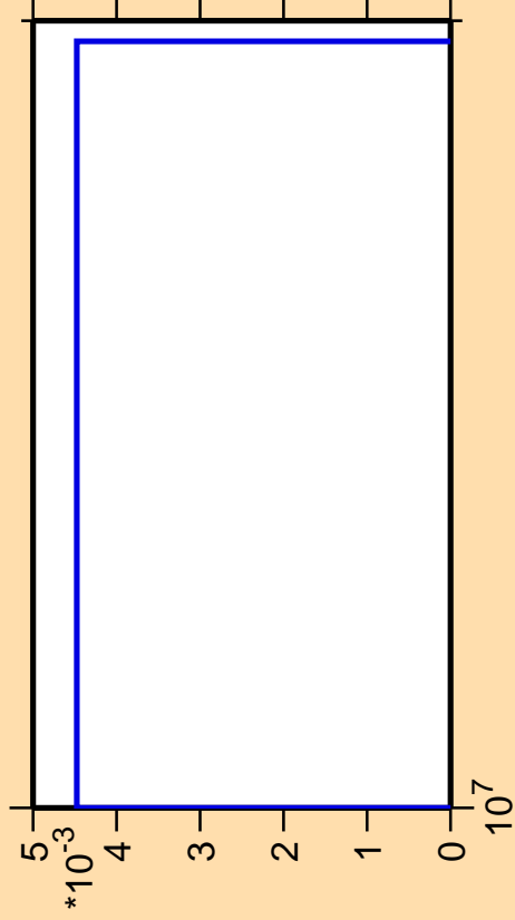
\Delta\sigma/\sigma vs. E for ^{222}\text{Po} (mt 11)
