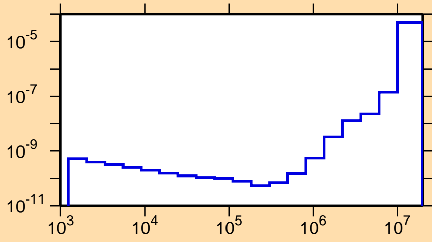
\sigma vs. E for ^{222}\text{Po}(n,\alpha)
