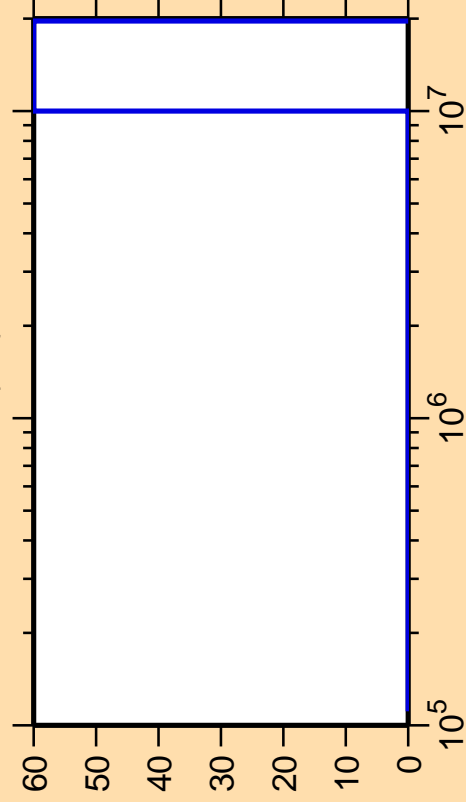
\Delta\sigma/\sigma vs. E for ^{222}\text{Po}(n,f)
