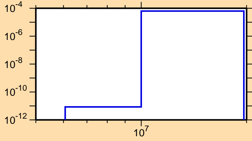
\sigma vs. E for ^{222}\text{Po}(n,p)
