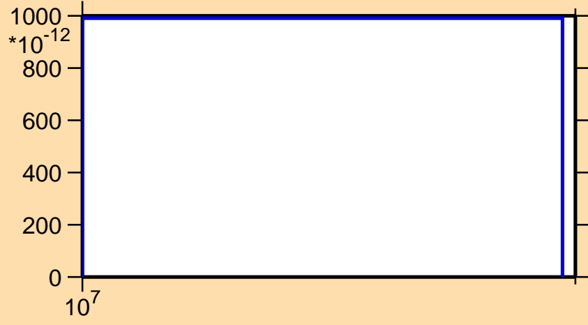
\sigma vs. E for ^{222}\text{Po}(n,\text{nd})
