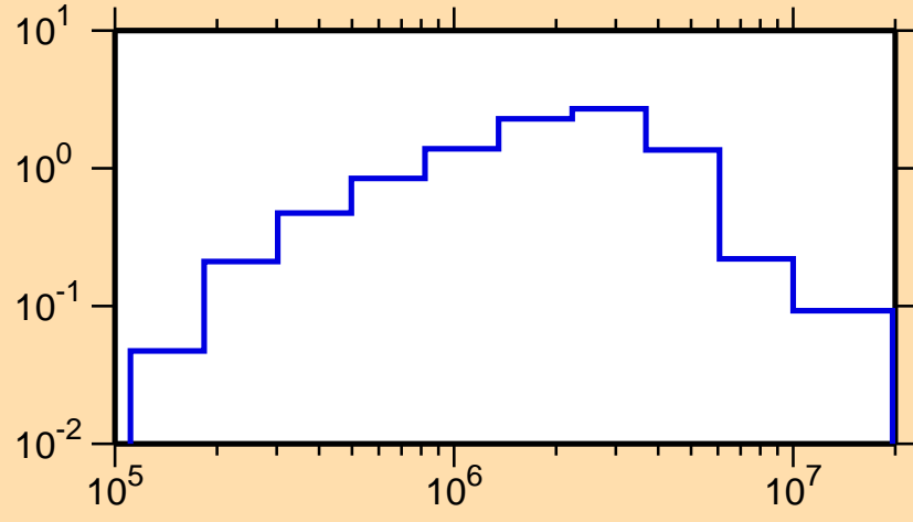
\sigma vs. E for ^{223}\text{Po}(n,\text{inel.})
