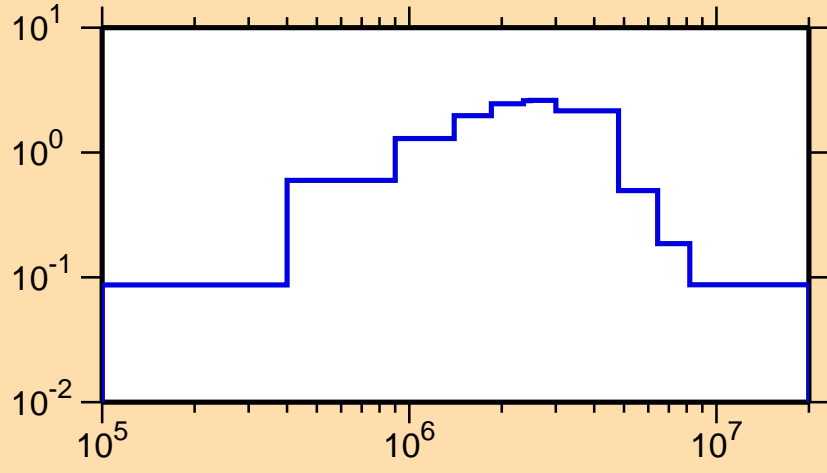
\sigma vs. E for ^{223}\text{Po}(n,n\text{cont.})
