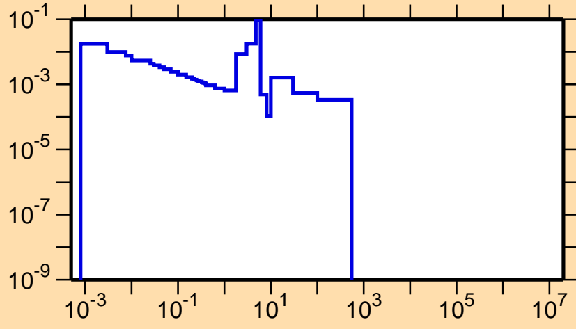
\sigma vs. E for ^{223}\text{Po}(n,f)
