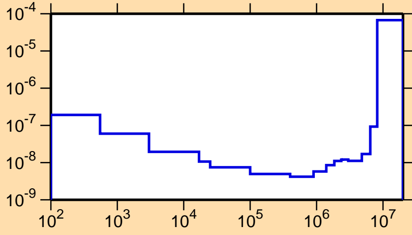
\sigma vs. E for ^{223}\text{Po}(n,\alpha)
