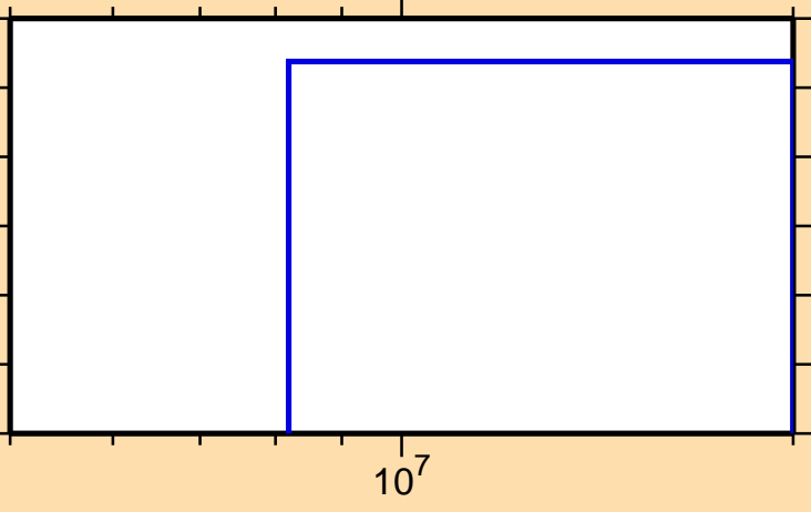
\sigma vs. E for ^{223}\text{Po}(n,t)
