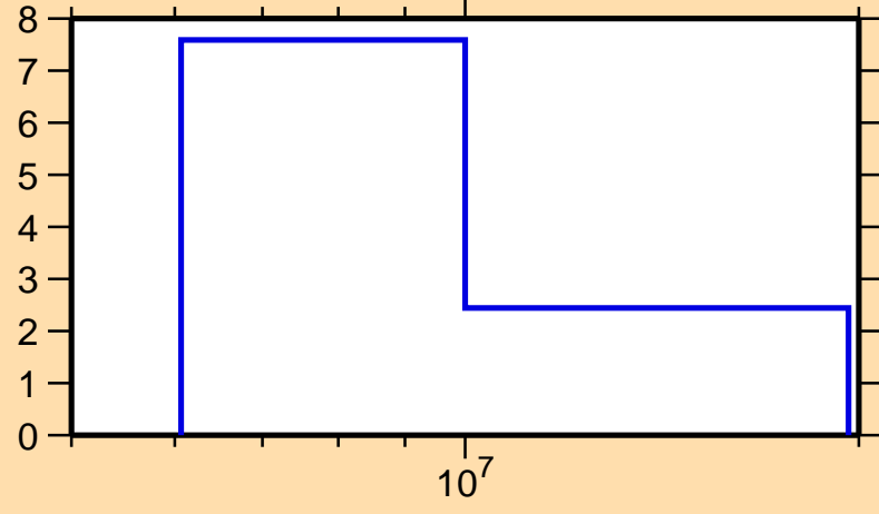
\Delta\sigma/\sigma vs. E for ^{224}\text{Po}(n,\text{nonel.})
