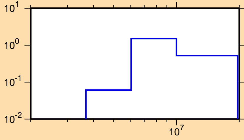
\sigma vs. E for ^{224}\text{Po}(n,2n)
