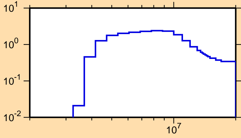
\sigma vs. E for ^{225}\text{Po}(n,2n)
