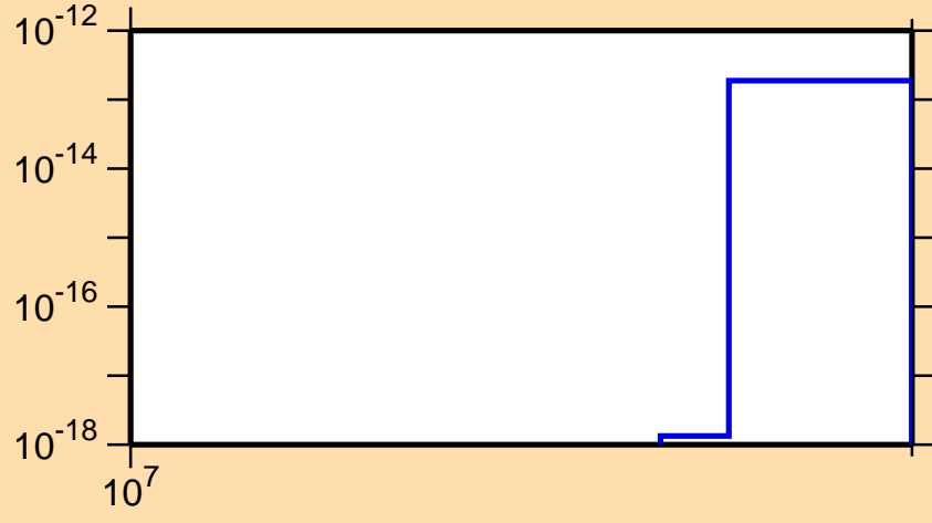
\sigma vs. E for ^{225}\text{Po} (mt 11)
