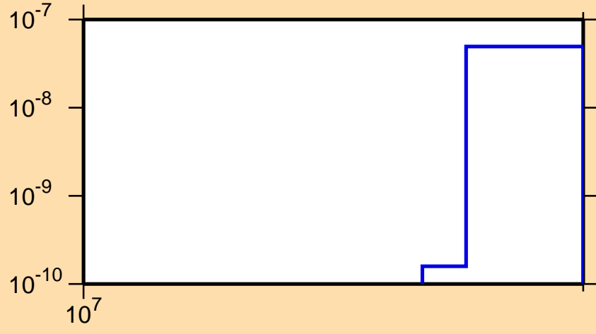
\sigma vs. E for ^{225}\text{Po}(n,2np)
