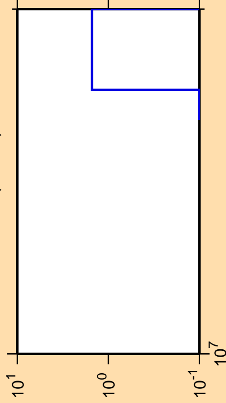
\Delta\sigma/\sigma vs. E for ^{225}\text{Po} (mt 11)
