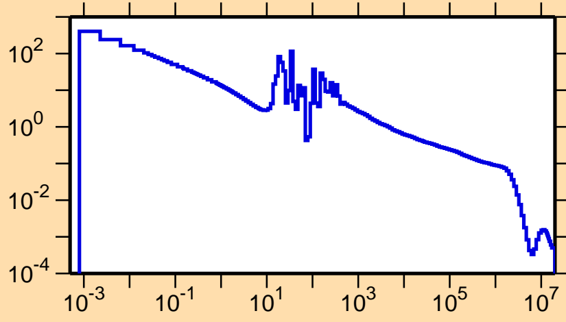
\sigma vs. E for ^{225}\text{Po}(n,\gamma)
