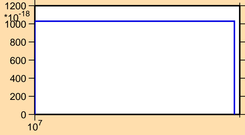
\sigma vs. E for ^{225}\text{Po} (mt 11)
