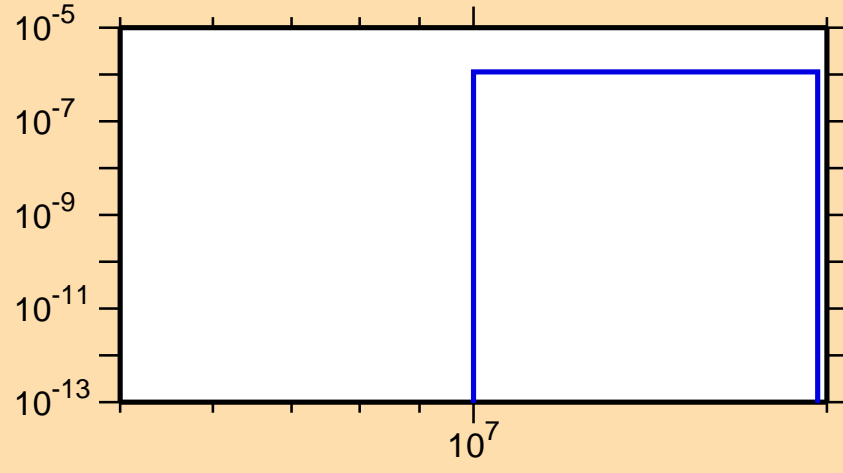
\sigma vs. E for ^{225}\text{Po}(n,np)
