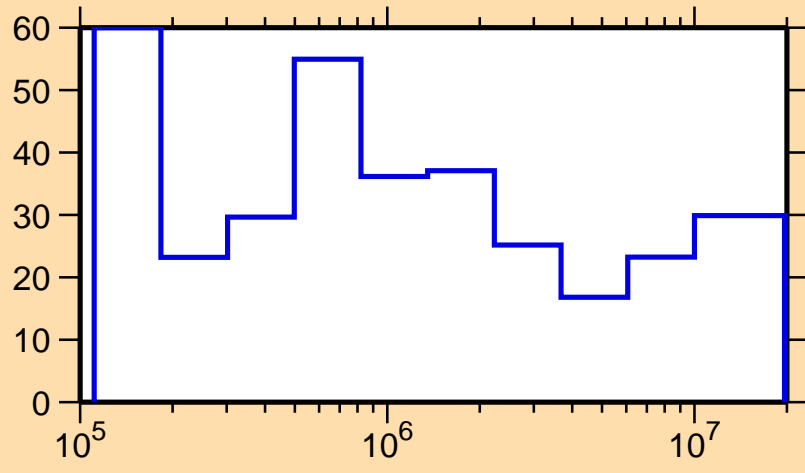
\Delta\sigma/\sigma vs. E for ^{225}\text{Po}(n,\text{nonel.})
