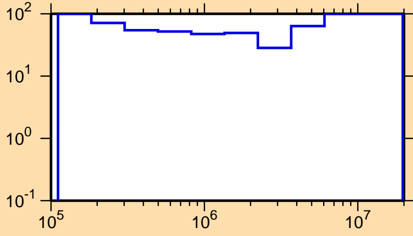
\Delta\sigma/\sigma vs. E for ^{225}\text{Po}(n,n\text{cont.})
