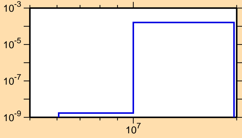
\sigma vs. E for ^{225}\text{Po}(n,p)
