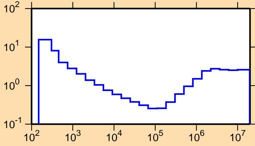
\sigma vs. E for ^{225}\text{Po}(n,\text{nonel.})
