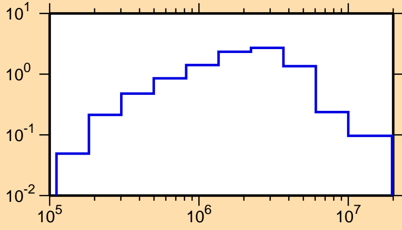
\sigma vs. E for ^{225}\text{Po}(n,\text{inel.})
