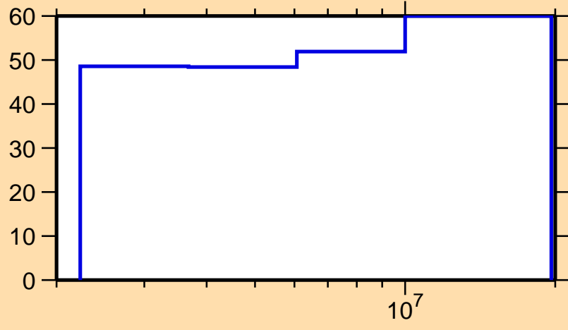
\Delta\sigma/\sigma vs. E for ^{225}\text{Po}(n,2n)
