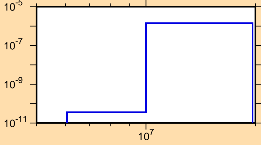
\sigma vs. E for ^{225}\text{Po}(n,n\alpha)
