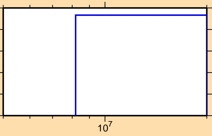
\sigma vs. E for ^{225}\text{Po}(n,np)
