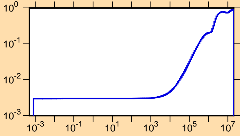
\mu vs. E for ^{226}\text{Po}(\text{mt251})
