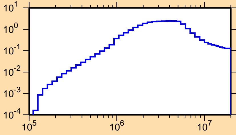
\sigma vs. E for ^{226}\text{Po}(n,n\text{cont.})
