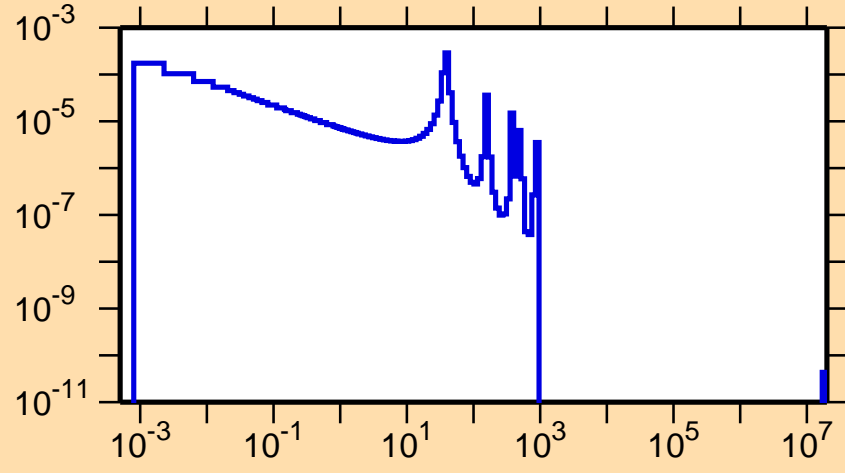
\sigma vs. E for ^{226}\text{Po}(n,f)
